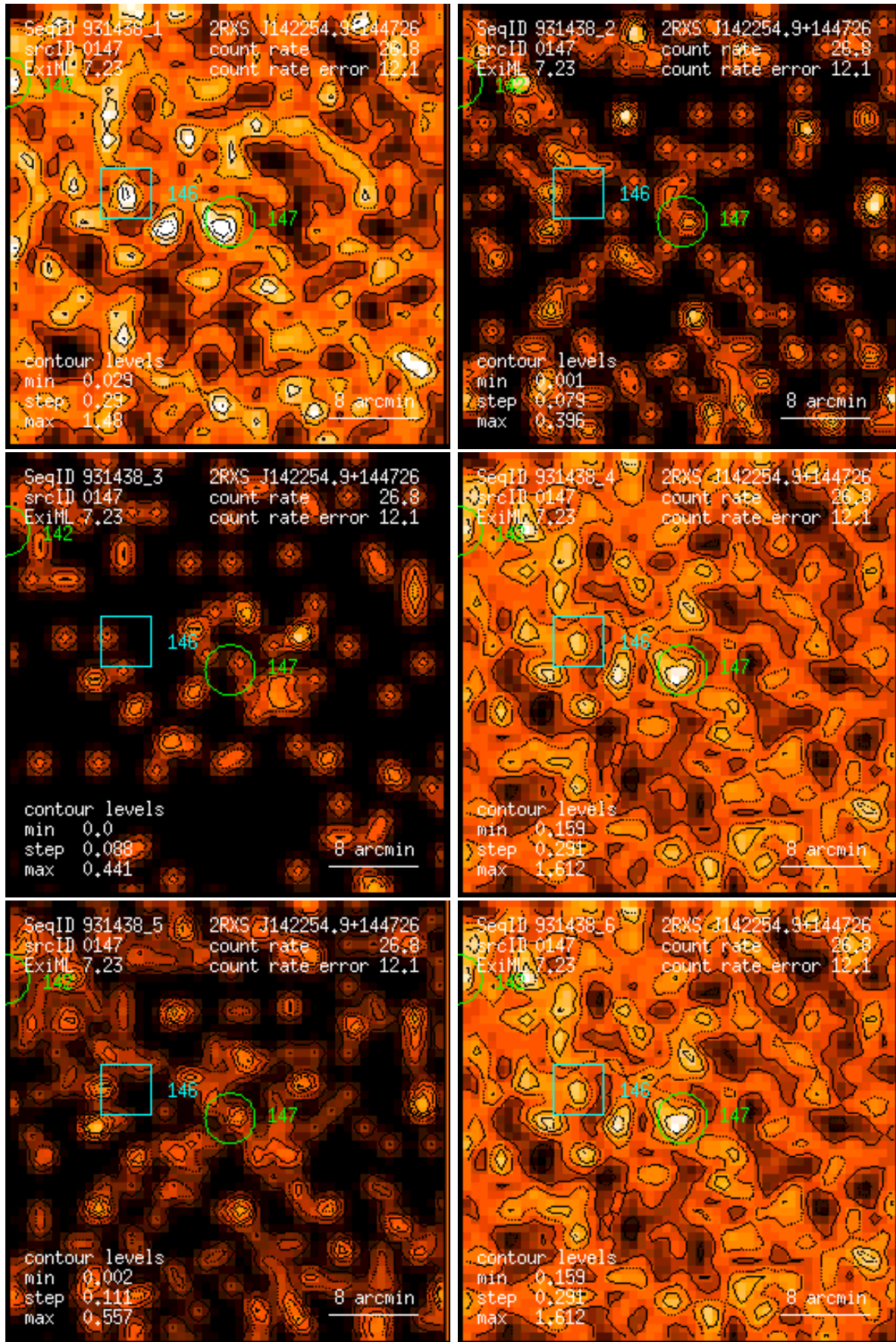
Figure 147: RASS 931438: detection 0147: band rate images, Gaussian filter: (1) PSPC channels 11 – 41, (2) 52 – 90, (3) 91 – 201, (4) 11 – 235, (5) 52 – 201, (6) 11 – 201. Broad band rates in counts/ks. Band rate contour levels in counts/ks/arcmin 2 .
