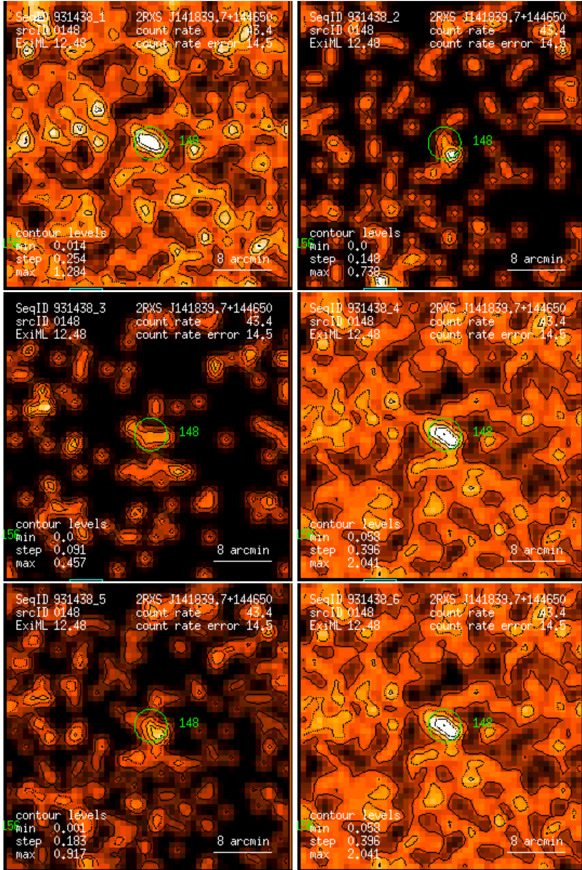
Figure 148: RASS 931438: detection 0148: band rate images, Gaussian filter: (1) PSPC channels 11 – 41, (2) 52 – 90, (3) 91 – 201, (4) 11 – 235, (5) 52 – 201, (6) 11 – 201. Broad band rates in counts/ks. Band rate contour levels in counts/ks/arcmin 2 .
