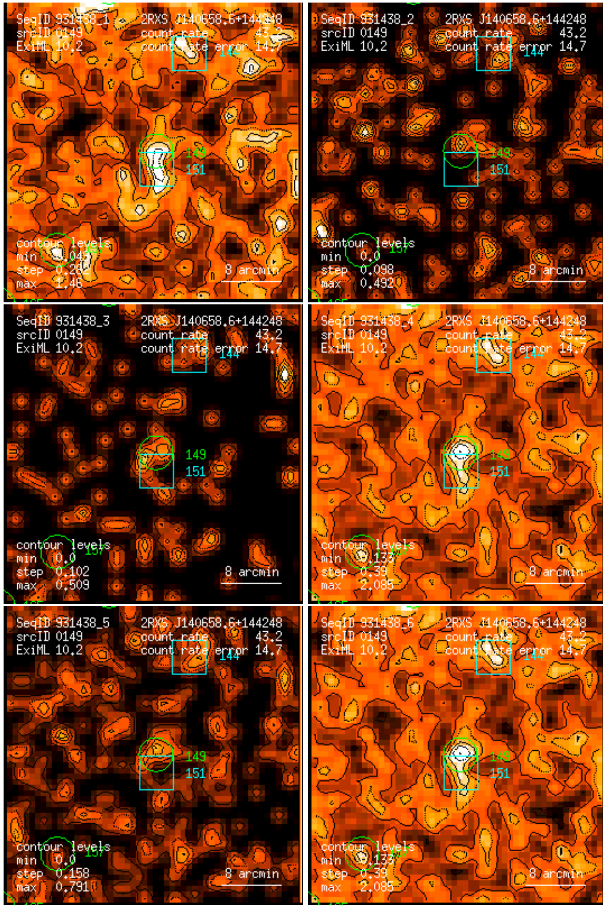
Figure 149: RASS 931438: detection 0149: band rate images, Gaussian filter: (1) PSPC channels 11 – 41, (2) 52 – 90, (3) 91 – 201, (4) 11 – 235, (5) 52 – 201, (6) 11 – 201. Broad band rates in counts/ks. Band rate contour levels in counts/ks/arcmin 2 .
