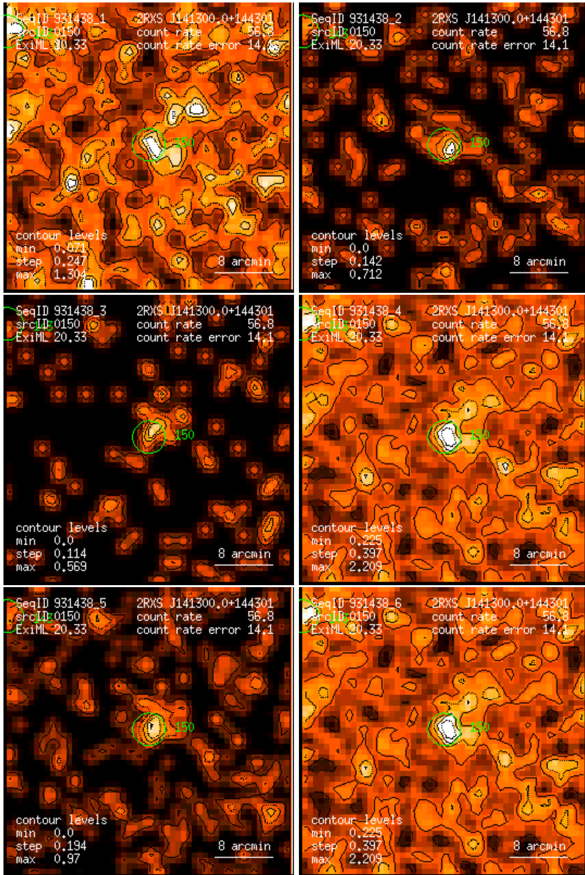
Figure 150: RASS 931438: detection 0150: band rate images, Gaussian filter: (1) PSPC channels 11 – 41, (2) 52 – 90, (3) 91 – 201, (4) 11 – 235, (5) 52 – 201, (6) 11 – 201. Broad band rates in counts/ks. Band rate contour levels in counts/ks/arcmin 2 .
