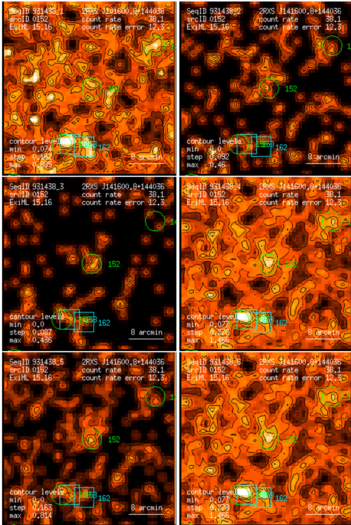
Figure 152: RASS 931438: detection 0152: band rate images, Gaussian filter: (1) PSPC channels 11 – 41, (2) 52 – 90, (3) 91 – 201, (4) 11 – 235, (5) 52 – 201, (6) 11 – 201. Broad band rates in counts/ks. Band rate contour levels in counts/ks/arcmin 2 .
