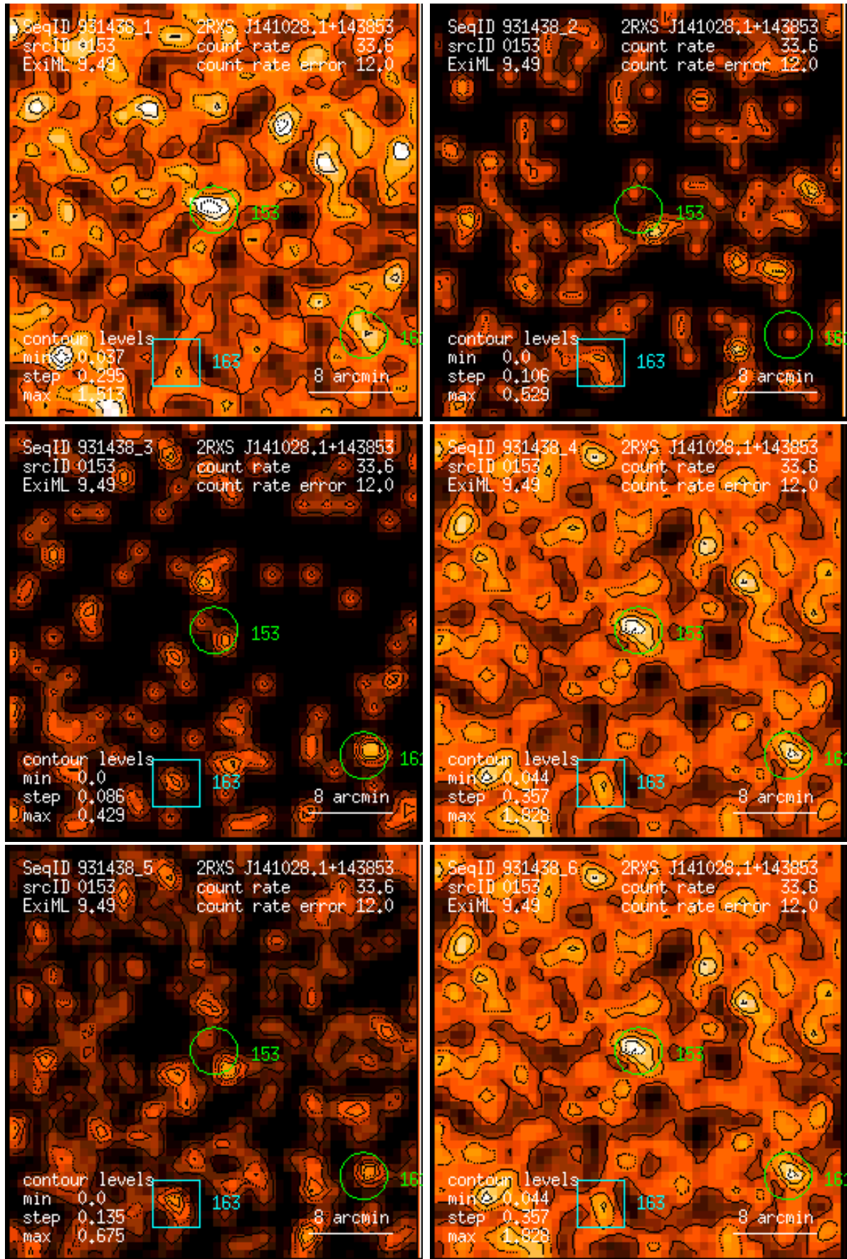
Figure 153: RASS 931438: detection 0153: band rate images, Gaussian filter: (1) PSPC channels 11 – 41, (2) 52 – 90, (3) 91 – 201, (4) 11 – 235, (5) 52 – 201, (6) 11 – 201. Broad band rates in counts/ks. Band rate contour levels in counts/ks/arcmin 2 .
