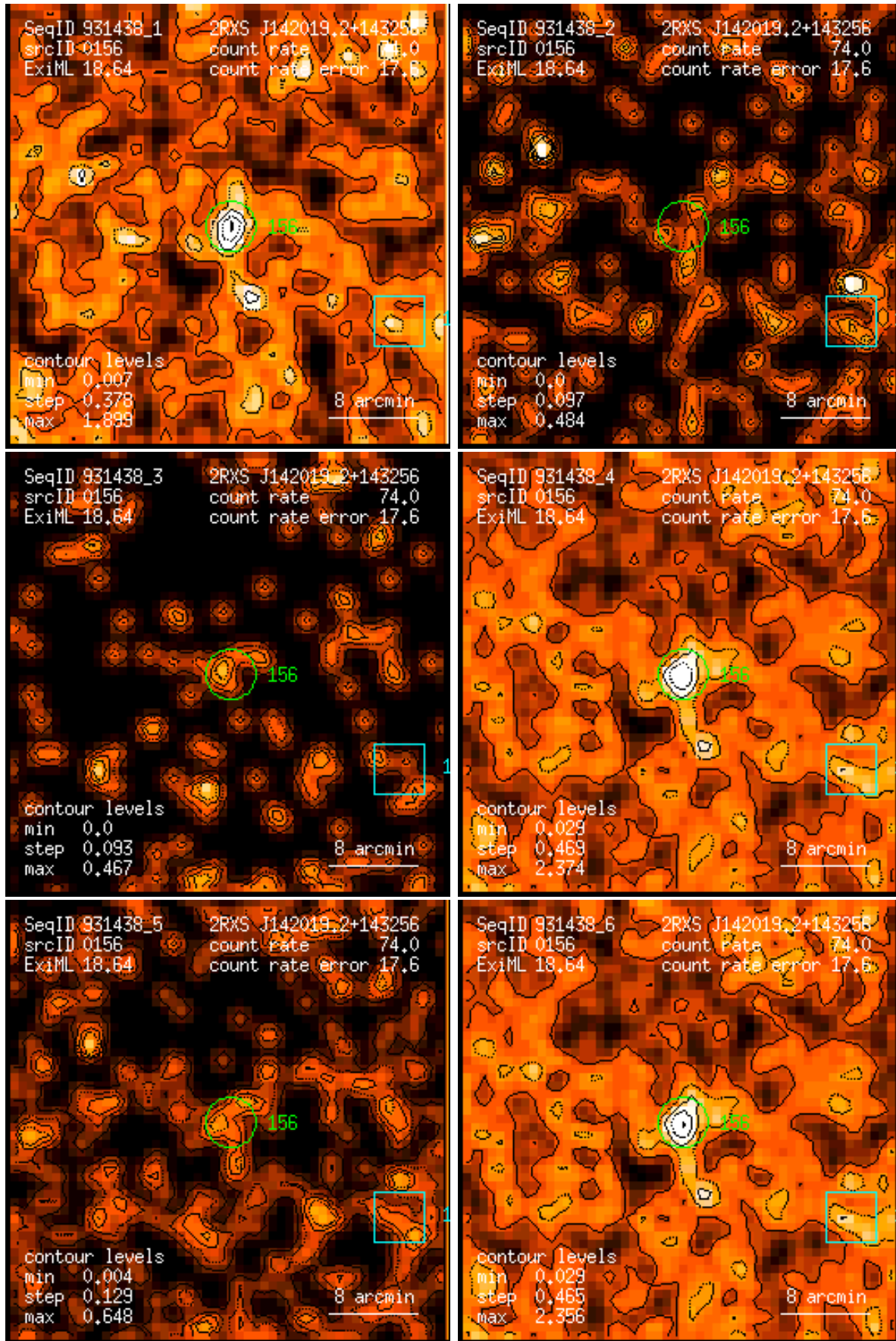
Figure 156: RASS 931438: detection 0156: band rate images, Gaussian filter: (1) PSPC channels 11 – 41, (2) 52 – 90, (3) 91 – 201, (4) 11 – 235, (5) 52 – 201, (6) 11 – 201. Broad band rates in counts/ks. Band rate contour levels in counts/ks/arcmin 2 .
