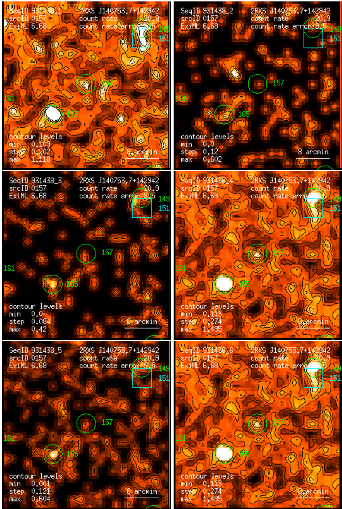
Figure 157: RASS 931438: detection 0157: band rate images, Gaussian filter: (1) PSPC channels 11 – 41, (2) 52 – 90, (3) 91 – 201, (4) 11 – 235, (5) 52 – 201, (6) 11 – 201. Broad band rates in counts/ks. Band rate contour levels in counts/ks/arcmin 2 .
