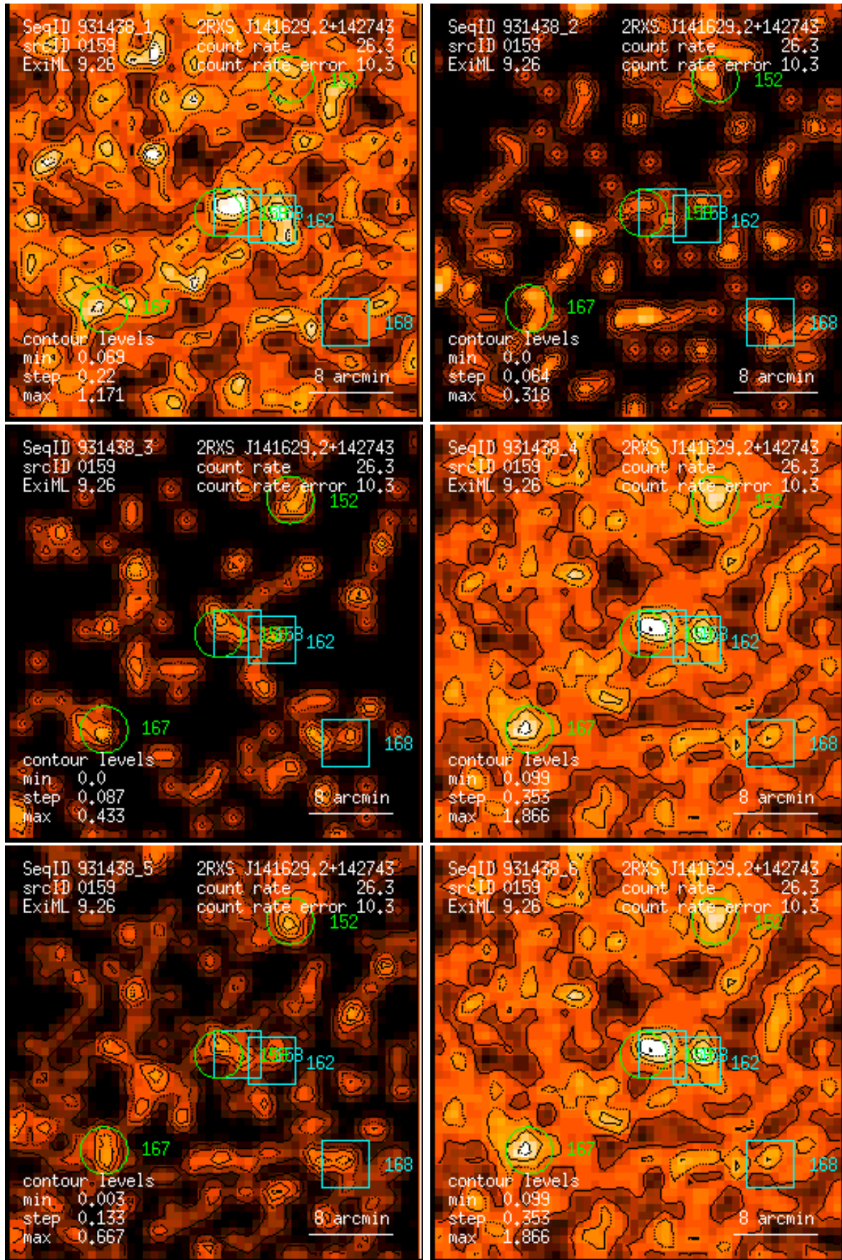
Figure 159: RASS 931438: detection 0159: band rate images, Gaussian filter: (1) PSPC channels 11 – 41, (2) 52 – 90, (3) 91 – 201, (4) 11 – 235, (5) 52 – 201, (6) 11 – 201. Broad band rates in counts/ks. Band rate contour levels in counts/ks/arcmin 2 .
