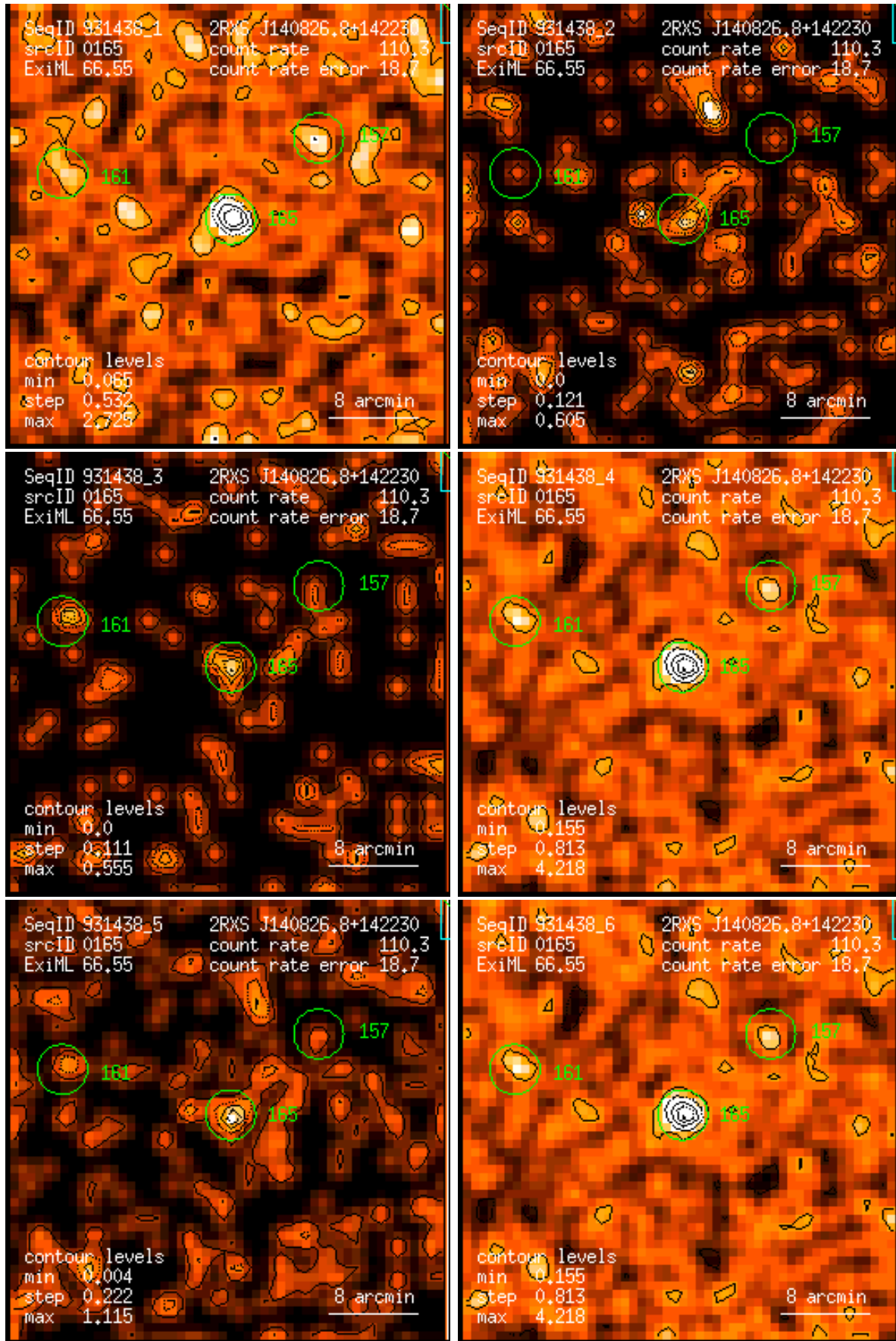
Figure 165: RASS 931438: detection 0165: band rate images, Gaussian filter: (1) PSPC channels 11 – 41, (2) 52 – 90, (3) 91 – 201, (4) 11 – 235, (5) 52 – 201, (6) 11 – 201. Broad band rates in counts/ks. Band rate contour levels in counts/ks/arcmin 2 .
