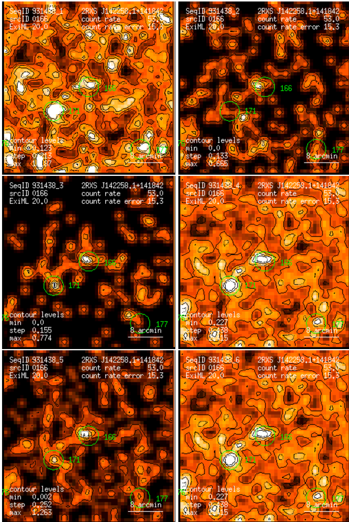
Figure 166: RASS 931438: detection 0166: band rate images, Gaussian filter: (1) PSPC channels 11 – 41, (2) 52 – 90, (3) 91 – 201, (4) 11 – 235, (5) 52 – 201, (6) 11 – 201. Broad band rates in counts/ks. Band rate contour levels in counts/ks/arcmin 2 .
