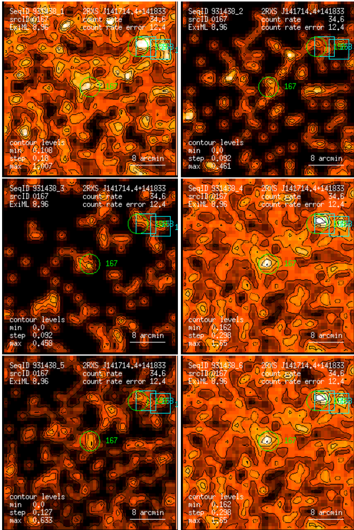
Figure 167: RASS 931438: detection 0167: band rate images, Gaussian filter: (1) PSPC channels 11 – 41, (2) 52 – 90, (3) 91 – 201, (4) 11 – 235, (5) 52 – 201, (6) 11 – 201. Broad band rates in counts/ks. Band rate contour levels in counts/ks/arcmin 2 .
