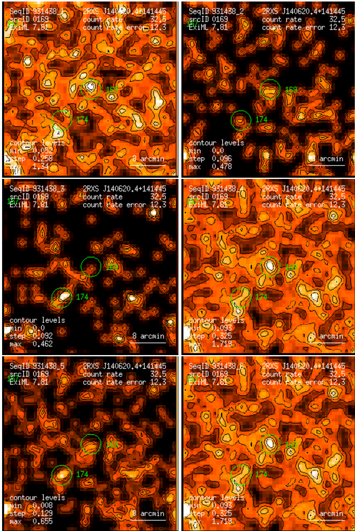
Figure 169: RASS 931438: detection 0169: band rate images, Gaussian filter: (1) PSPC channels 11 – 41, (2) 52 – 90, (3) 91 – 201, (4) 11 – 235, (5) 52 – 201, (6) 11 – 201. Broad band rates in counts/ks. Band rate contour levels in counts/ks/arcmin 2 .
