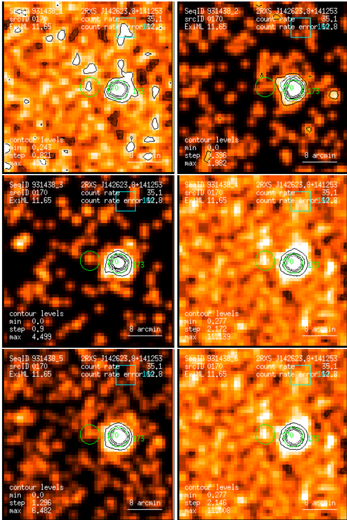
Figure 170: RASS 931438: detection 0170: band rate images, Gaussian filter: (1) PSPC channels 11 – 41, (2) 52 – 90, (3) 91 – 201, (4) 11 – 235, (5) 52 – 201, (6) 11 – 201. Broad band rates in counts/ks. Band rate contour levels in counts/ks/arcmin 2 .
