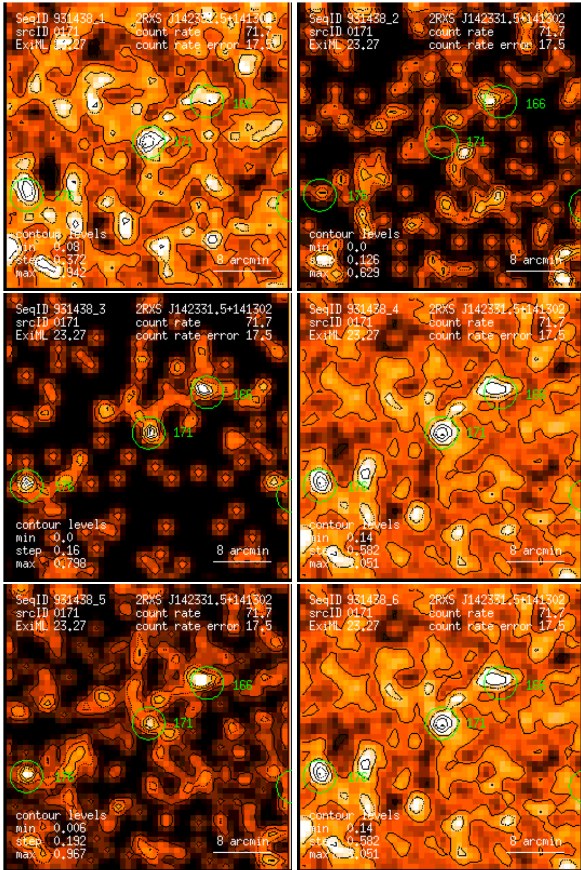
Figure 171: RASS 931438: detection 0171: band rate images, Gaussian filter: (1) PSPC channels 11 – 41, (2) 52 – 90, (3) 91 – 201, (4) 11 – 235, (5) 52 – 201, (6) 11 – 201. Broad band rates in counts/ks. Band rate contour levels in counts/ks/arcmin 2 .
