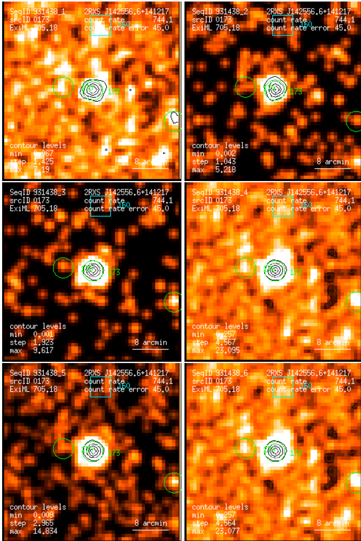
Figure 173: RASS 931438: detection 0173: band rate images, Gaussian filter: (1) PSPC channels 11 – 41, (2) 52 – 90, (3) 91 – 201, (4) 11 – 235, (5) 52 – 201, (6) 11 – 201. Broad band rates in counts/ks. Band rate contour levels in counts/ks/arcmin 2 .
