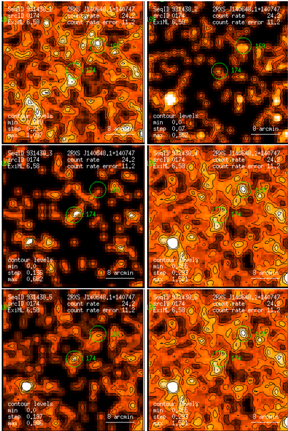
Figure 174: RASS 931438: detection 0174: band rate images, Gaussian filter: (1) PSPC channels 11 – 41, (2) 52 – 90, (3) 91 – 201, (4) 11 – 235, (5) 52 – 201, (6) 11 – 201. Broad band rates in counts/ks. Band rate contour levels in counts/ks/arcmin 2 .
