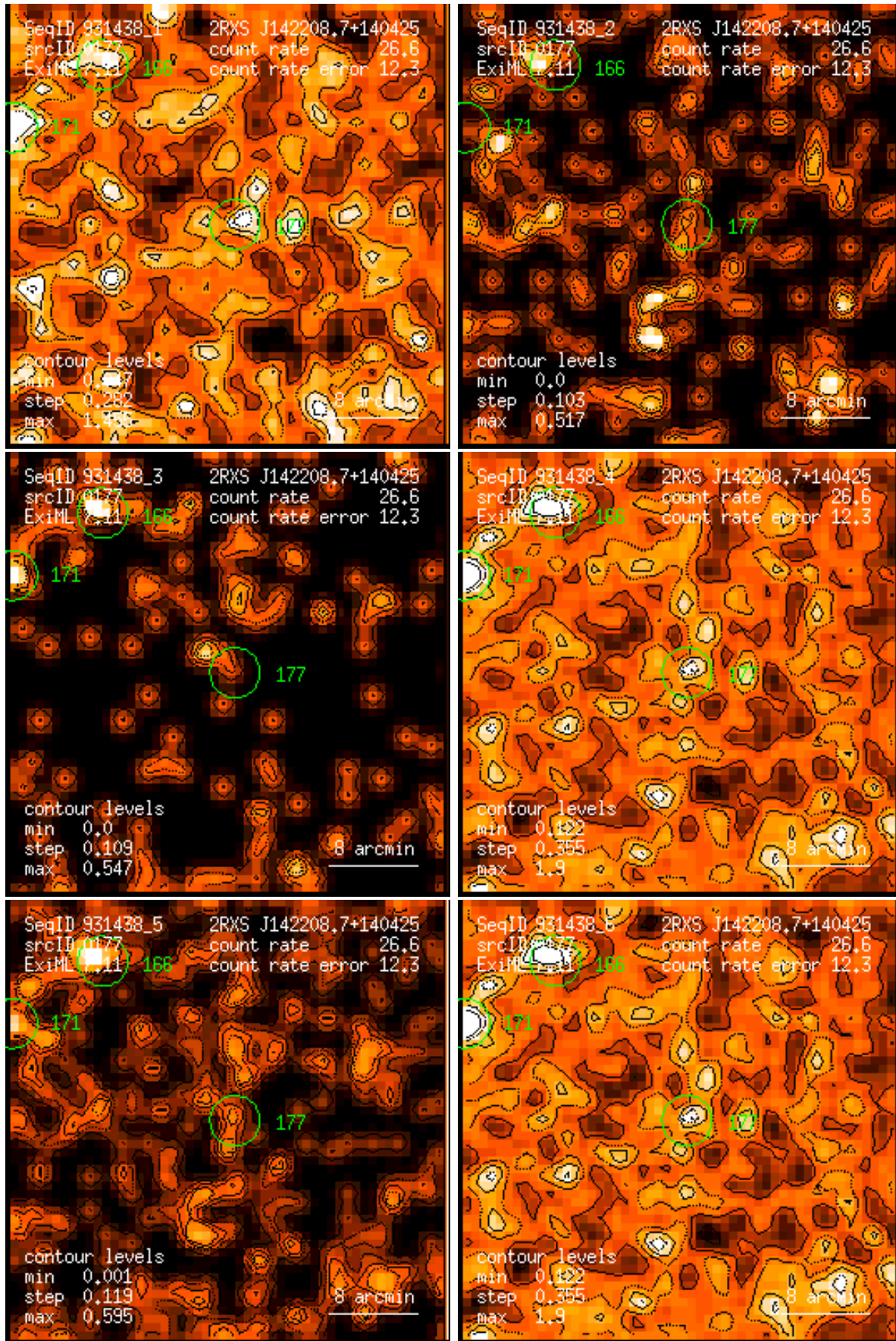
Figure 177: RASS 931438: detection 0177: band rate images, Gaussian filter: (1) PSPC channels 11 – 41, (2) 52 – 90, (3) 91 – 201, (4) 11 – 235, (5) 52 – 201, (6) 11 – 201. Broad band rates in counts/ks. Band rate contour levels in counts/ks/arcmin 2 .
