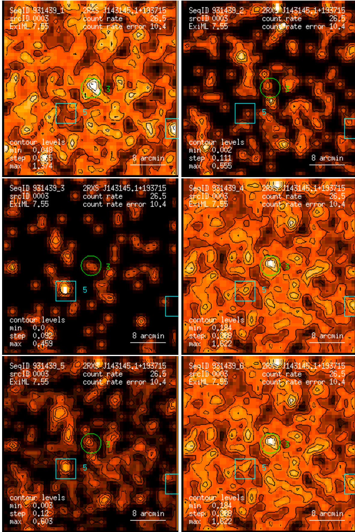
Figure 3: RASS 931439: detection 0003: band rate images, Gaussian filter: (1) PSPC channels 11 – 41, (2) 52 – 90, (3) 91 – 201, (4) 11 – 235, (5) 52 – 201, (6) 11 – 201. Broad band rates in counts/ks. Band rate contour levels in counts/ks/arcmin 2 .
