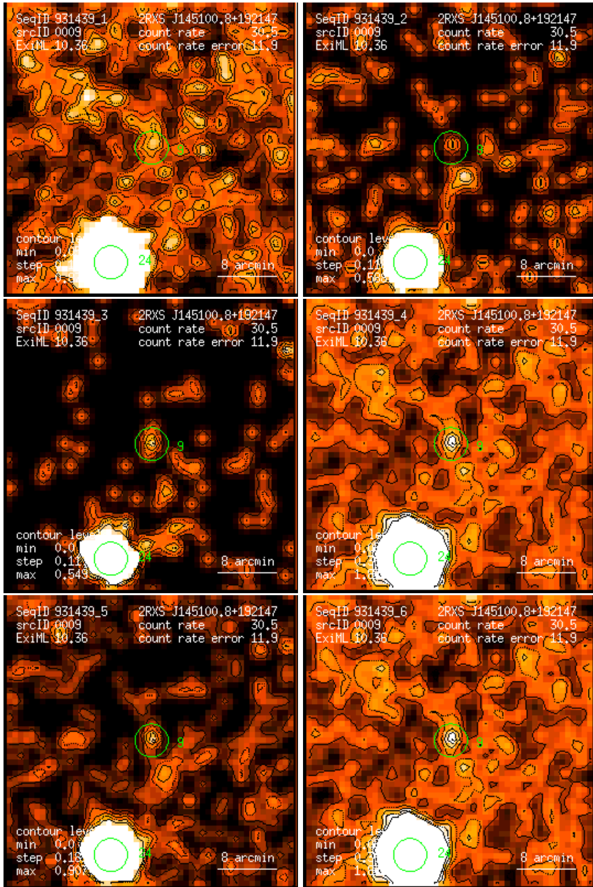
Figure 9: RASS 931439: detection 0009: band rate images, Gaussian filter: (1) PSPC channels 11 – 41, (2) 52 – 90, (3) 91 – 201, (4) 11 – 235, (5) 52 – 201, (6) 11 – 201. Broad band rates in counts/ks. Band rate contour levels in counts/ks/arcmin 2 .
