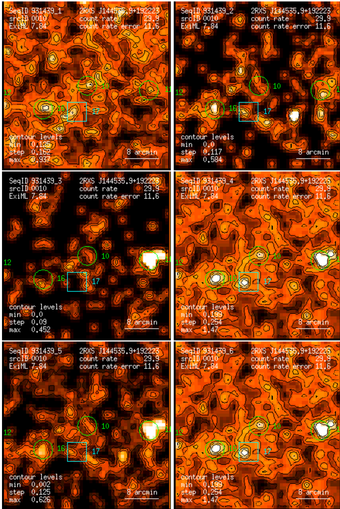
Figure 10: RASS 931439: detection 0010: band rate images, Gaussian filter: (1) PSPC channels 11 – 41, (2) 52 – 90, (3) 91 – 201, (4) 11 – 235, (5) 52 – 201, (6) 11 – 201. Broad band rates in counts/ks. Band rate contour levels in counts/ks/arcmin 2 .
