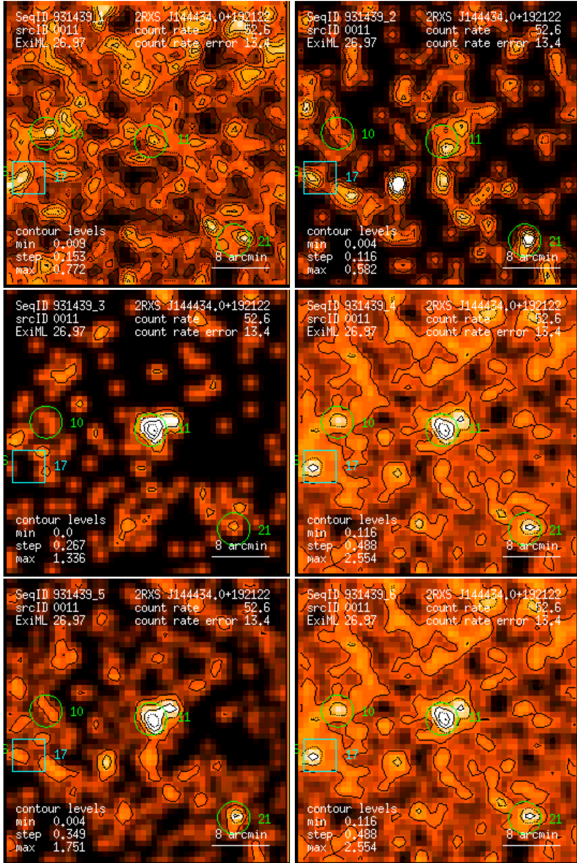
Figure 11: RASS 931439: detection 0011: band rate images, Gaussian filter: (1) PSPC channels 11 – 41, (2) 52 – 90, (3) 91 – 201, (4) 11 – 235, (5) 52 – 201, (6) 11 – 201. Broad band rates in counts/ks. Band rate contour levels in counts/ks/arcmin 2 .
