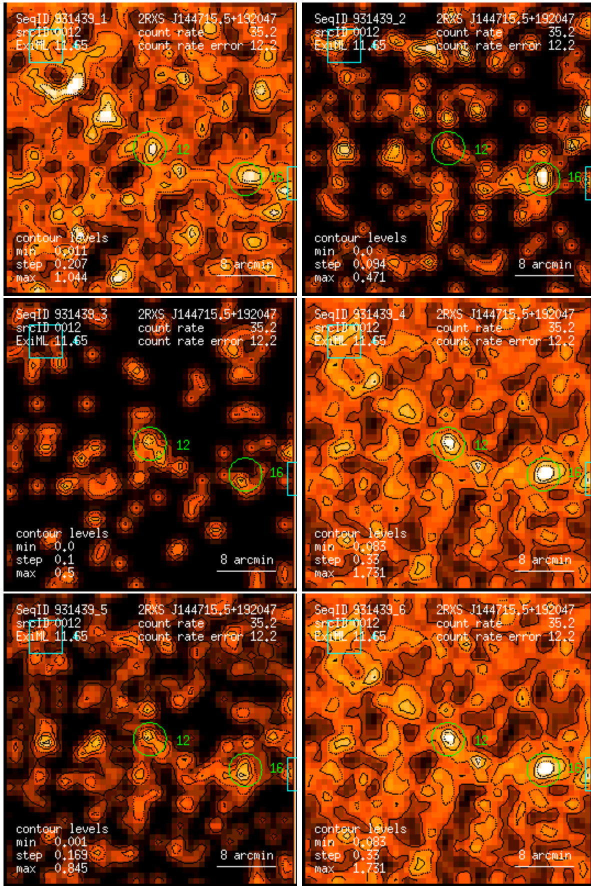
Figure 12: RASS 931439: detection 0012: band rate images, Gaussian filter: (1) PSPC channels 11 – 41, (2) 52 – 90, (3) 91 – 201, (4) 11 – 235, (5) 52 – 201, (6) 11 – 201. Broad band rates in counts/ks. Band rate contour levels in counts/ks/arcmin 2 .
