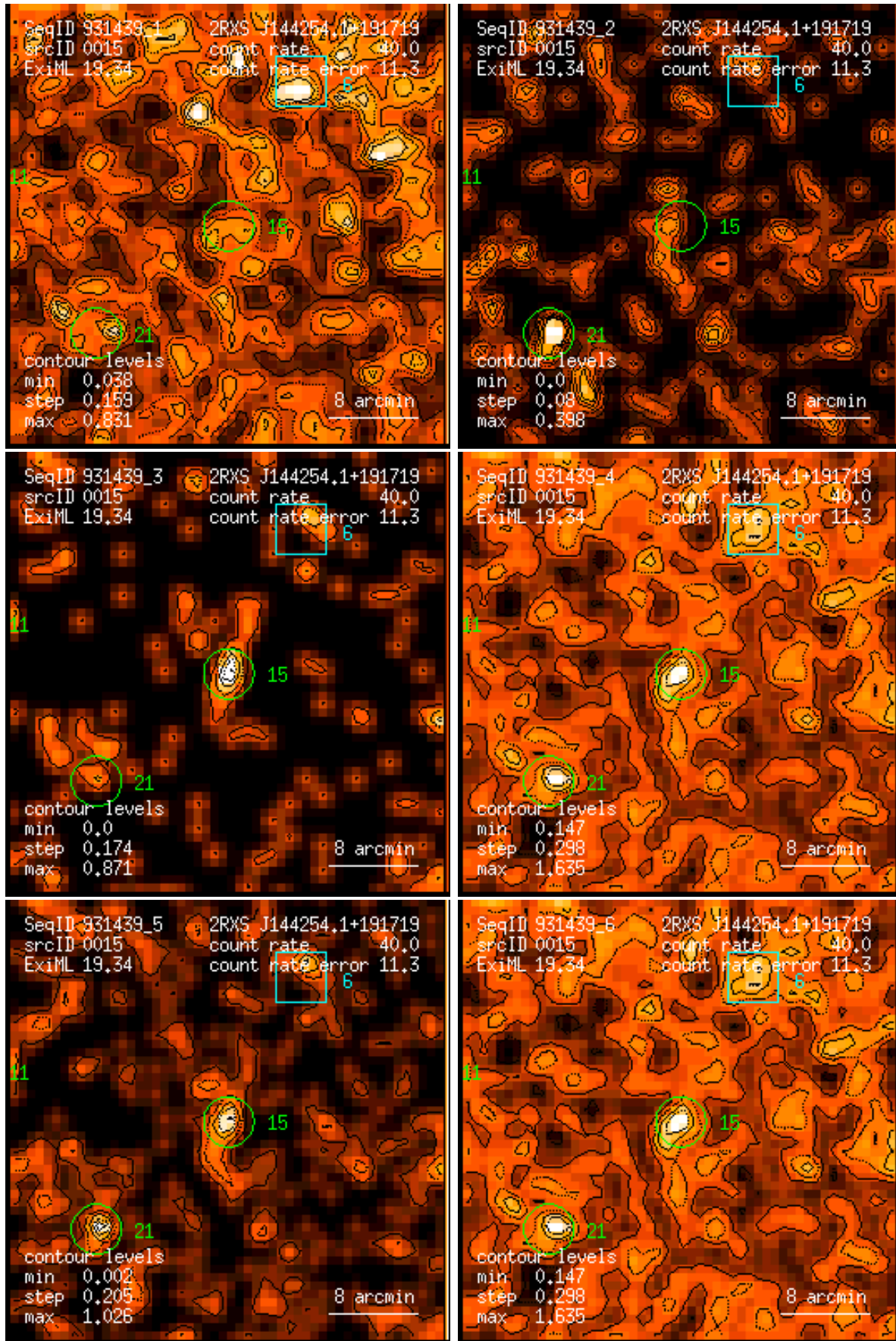
Figure 15: RASS 931439: detection 0015: band rate images, Gaussian filter: (1) PSPC channels 11 – 41, (2) 52 – 90, (3) 91 – 201, (4) 11 – 235, (5) 52 – 201, (6) 11 – 201. Broad band rates in counts/ks. Band rate contour levels in counts/ks/arcmin 2 .
