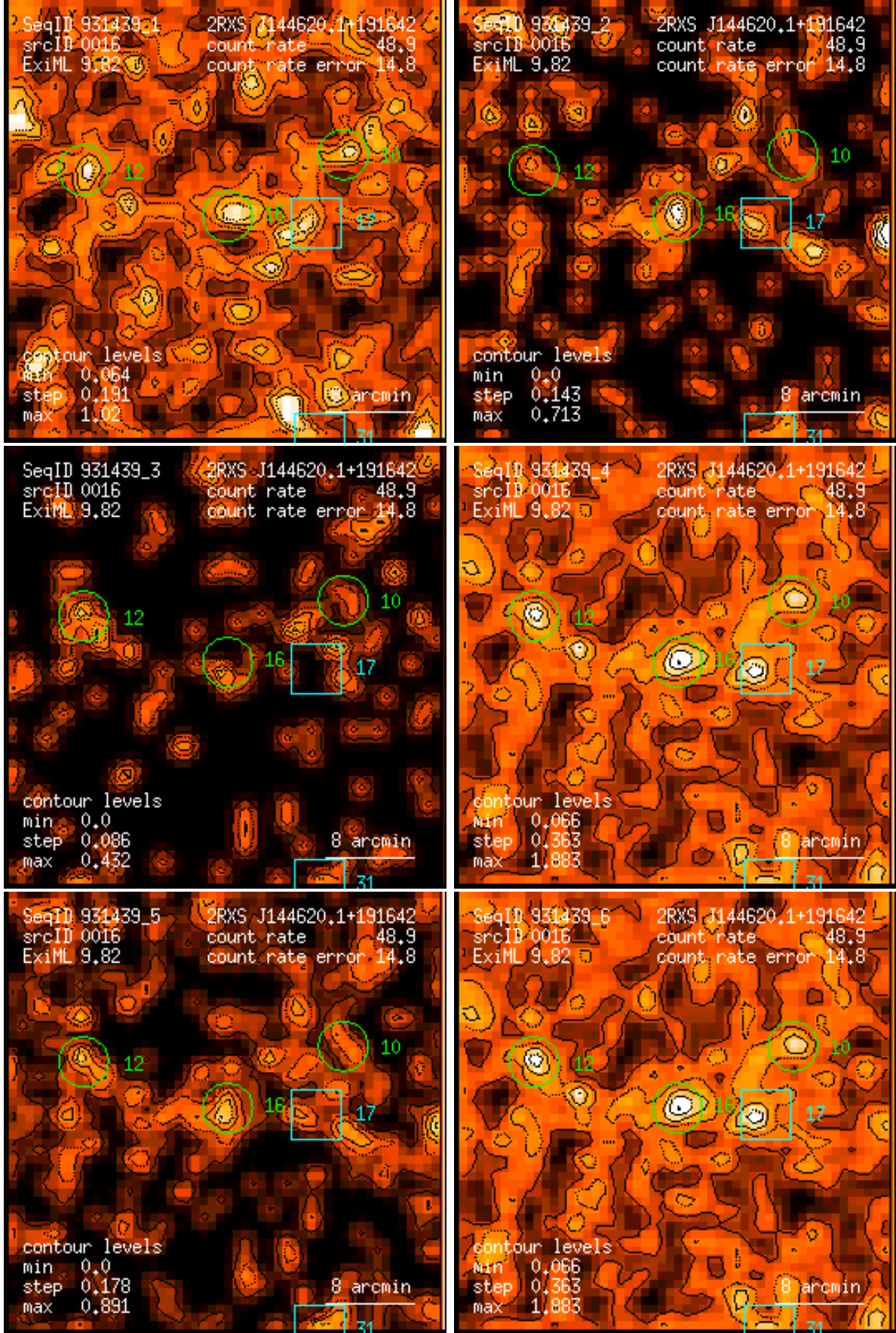
Figure 16: RASS 931439: detection 0016: band rate images, Gaussian filter: (1) PSPC channels 11 – 41, (2) 52 – 90, (3) 91 – 201, (4) 11 – 235, (5) 52 – 201, (6) 11 – 201. Broad band rates in counts/ks. Band rate contour levels in counts/ks/arcmin 2 .
