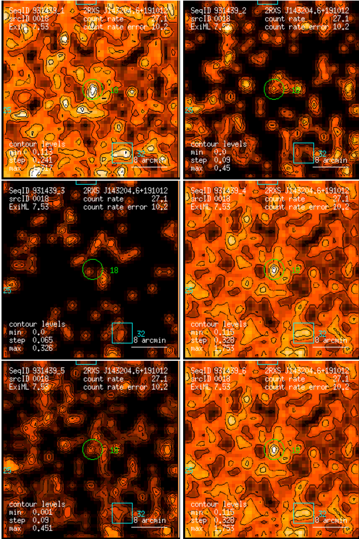
Figure 18: RASS 931439: detection 0018: band rate images, Gaussian filter: (1) PSPC channels 11 – 41, (2) 52 – 90, (3) 91 – 201, (4) 11 – 235, (5) 52 – 201, (6) 11 – 201. Broad band rates in counts/ks. Band rate contour levels in counts/ks/arcmin 2 .
