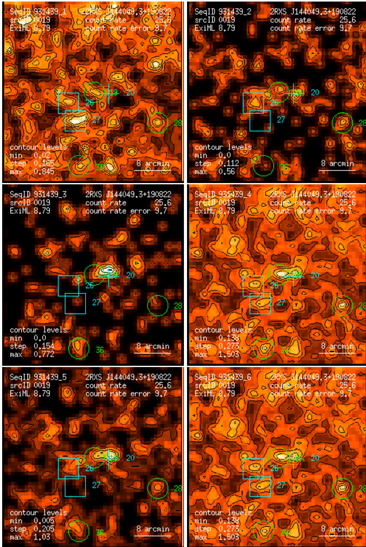
Figure 19: RASS 931439: detection 0019: band rate images, Gaussian filter: (1) PSPC channels 11 – 41, (2) 52 – 90, (3) 91 – 201, (4) 11 – 235, (5) 52 – 201, (6) 11 – 201. Broad band rates in counts/ks. Band rate contour levels in counts/ks/arcmin 2 .
