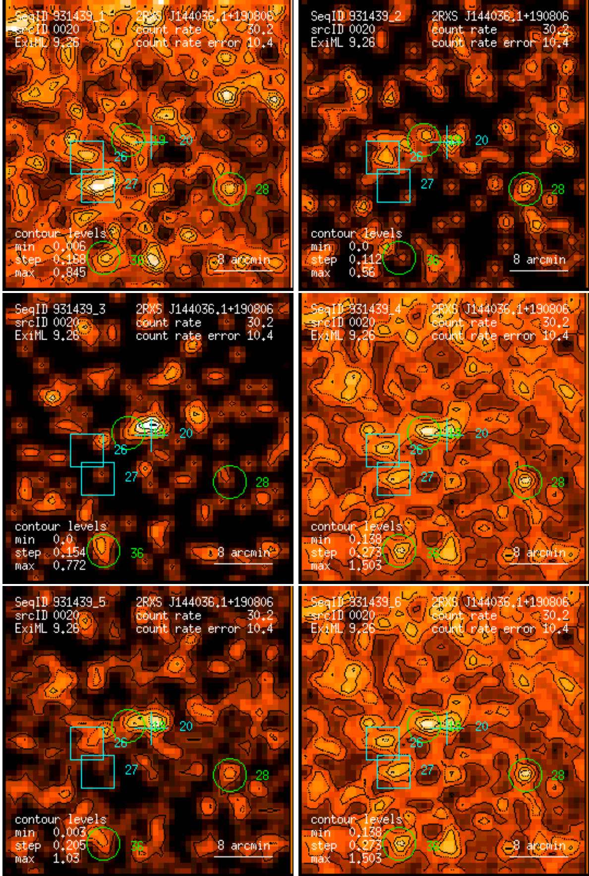
Figure 20: RASS 931439: detection 0020: band rate images, Gaussian filter: (1) PSPC channels 11 – 41, (2) 52 – 90, (3) 91 – 201, (4) 11 – 235, (5) 52 – 201, (6) 11 – 201. Broad band rates in counts/ks. Band rate contour levels in counts/ks/arcmin 2 .
