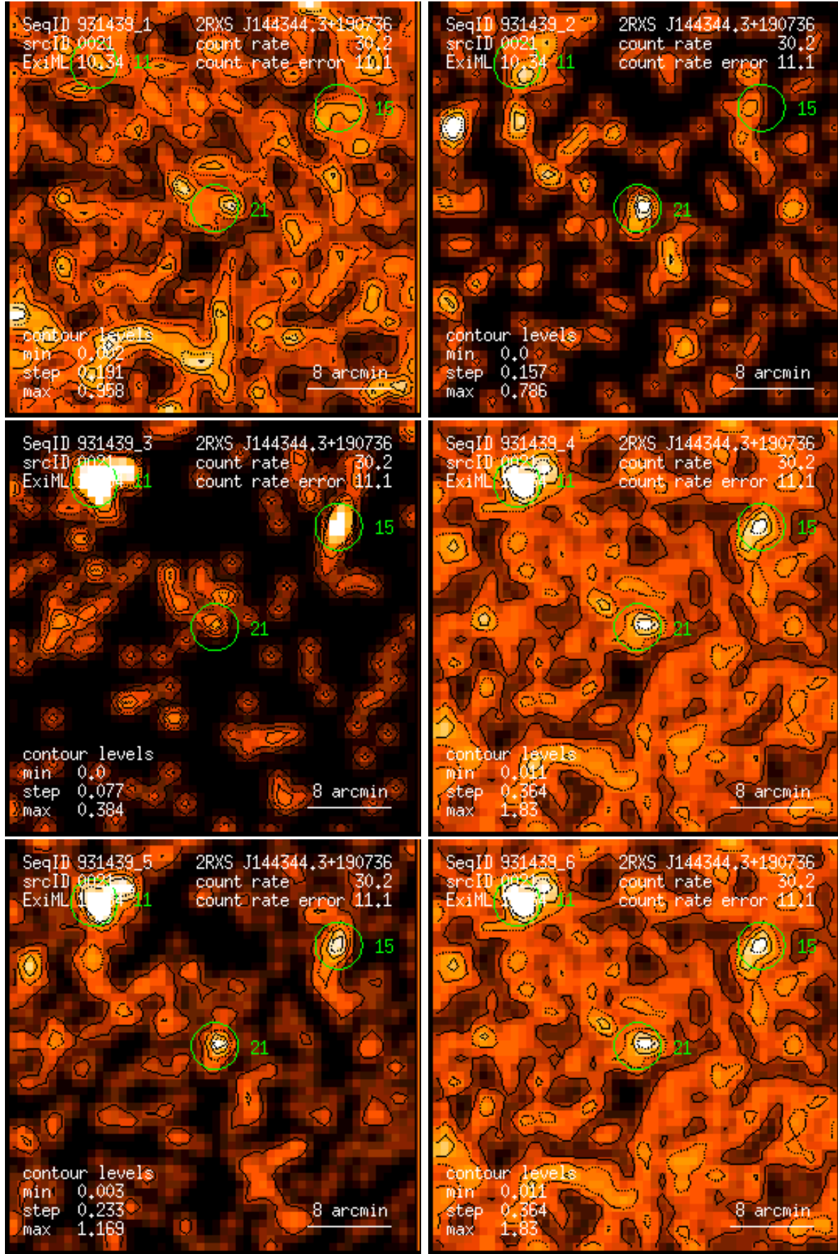
Figure 21: RASS 931439: detection 0021: band rate images, Gaussian filter: (1) PSPC channels 11 – 41, (2) 52 – 90, (3) 91 – 201, (4) 11 – 235, (5) 52 – 201, (6) 11 – 201. Broad band rates in counts/ks. Band rate contour levels in counts/ks/arcmin 2 .
