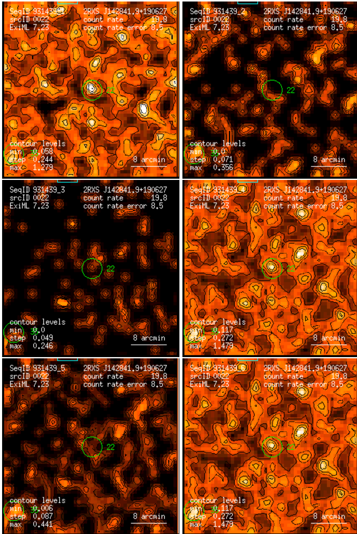
Figure 22: RASS 931439: detection 0022: band rate images, Gaussian filter: (1) PSPC channels 11 – 41, (2) 52 – 90, (3) 91 – 201, (4) 11 – 235, (5) 52 – 201, (6) 11 – 201. Broad band rates in counts/ks. Band rate contour levels in counts/ks/arcmin 2 .
