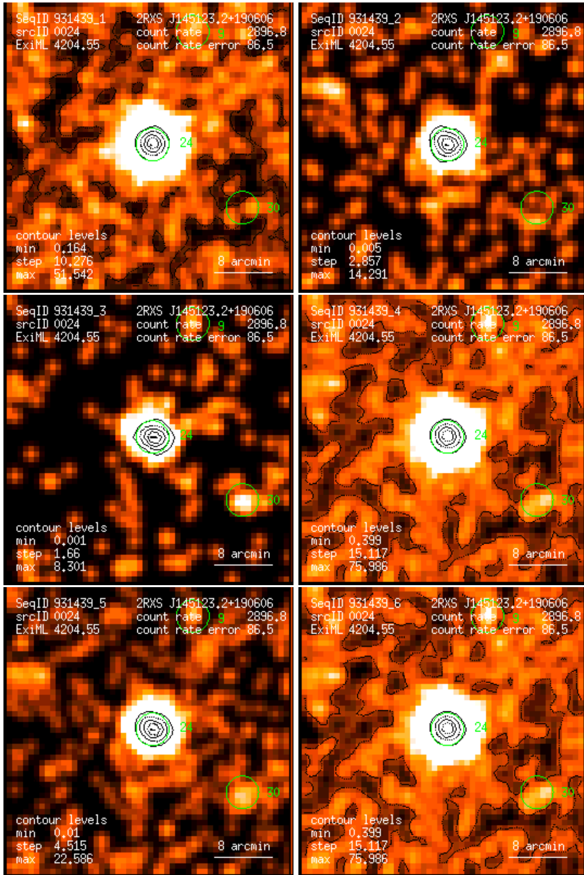
Figure 24: RASS 931439: detection 0024: band rate images, Gaussian filter: (1) PSPC channels 11 – 41, (2) 52 – 90, (3) 91 – 201, (4) 11 – 235, (5) 52 – 201, (6) 11 – 201. Broad band rates in counts/ks. Band rate contour levels in counts/ks/arcmin 2 .
