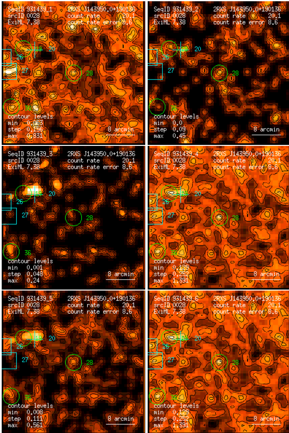
Figure 28: RASS 931439: detection 0028: band rate images, Gaussian filter: (1) PSPC channels 11 – 41, (2) 52 – 90, (3) 91 – 201, (4) 11 – 235, (5) 52 – 201, (6) 11 – 201. Broad band rates in counts/ks. Band rate contour levels in counts/ks/arcmin 2 .
