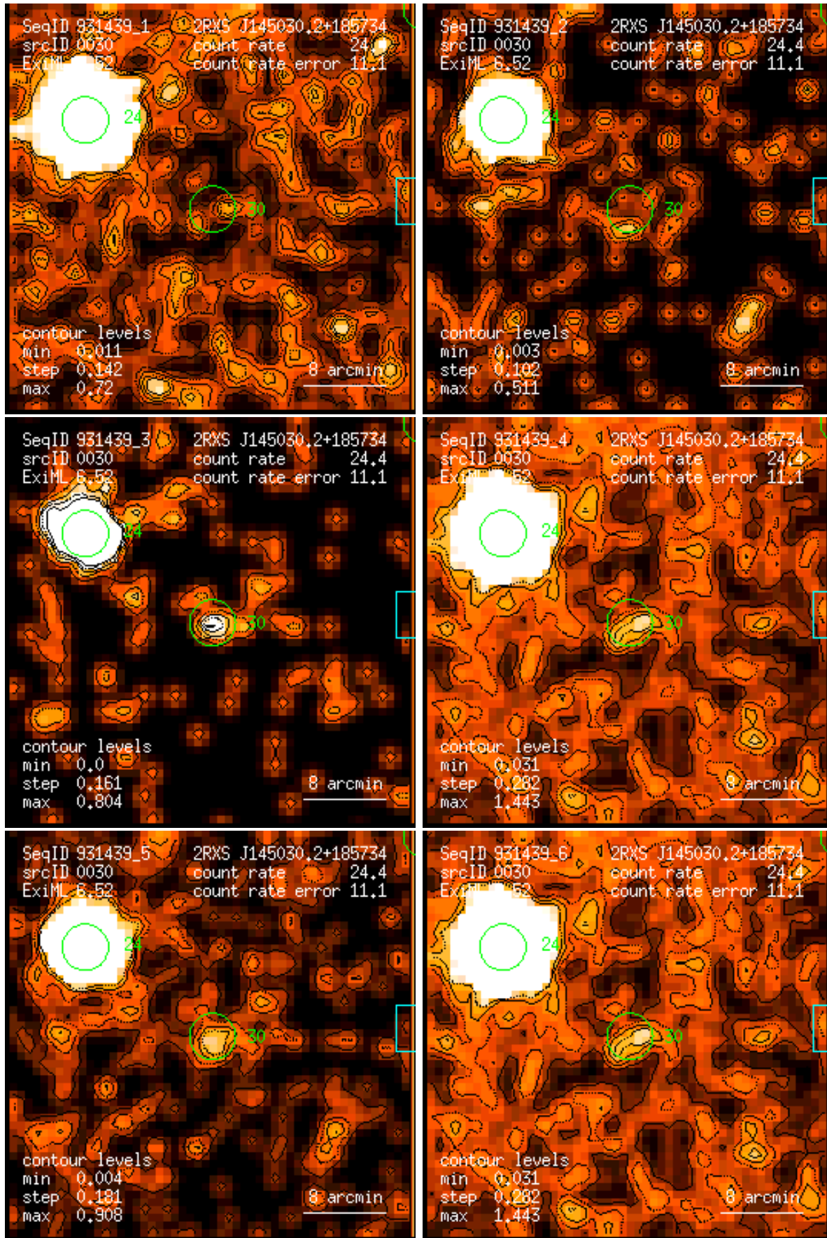
Figure 30: RASS 931439: detection 0030: band rate images, Gaussian filter: (1) PSPC channels 11 – 41, (2) 52 – 90, (3) 91 – 201, (4) 11 – 235, (5) 52 – 201, (6) 11 – 201. Broad band rates in counts/ks. Band rate contour levels in counts/ks/arcmin 2 .
