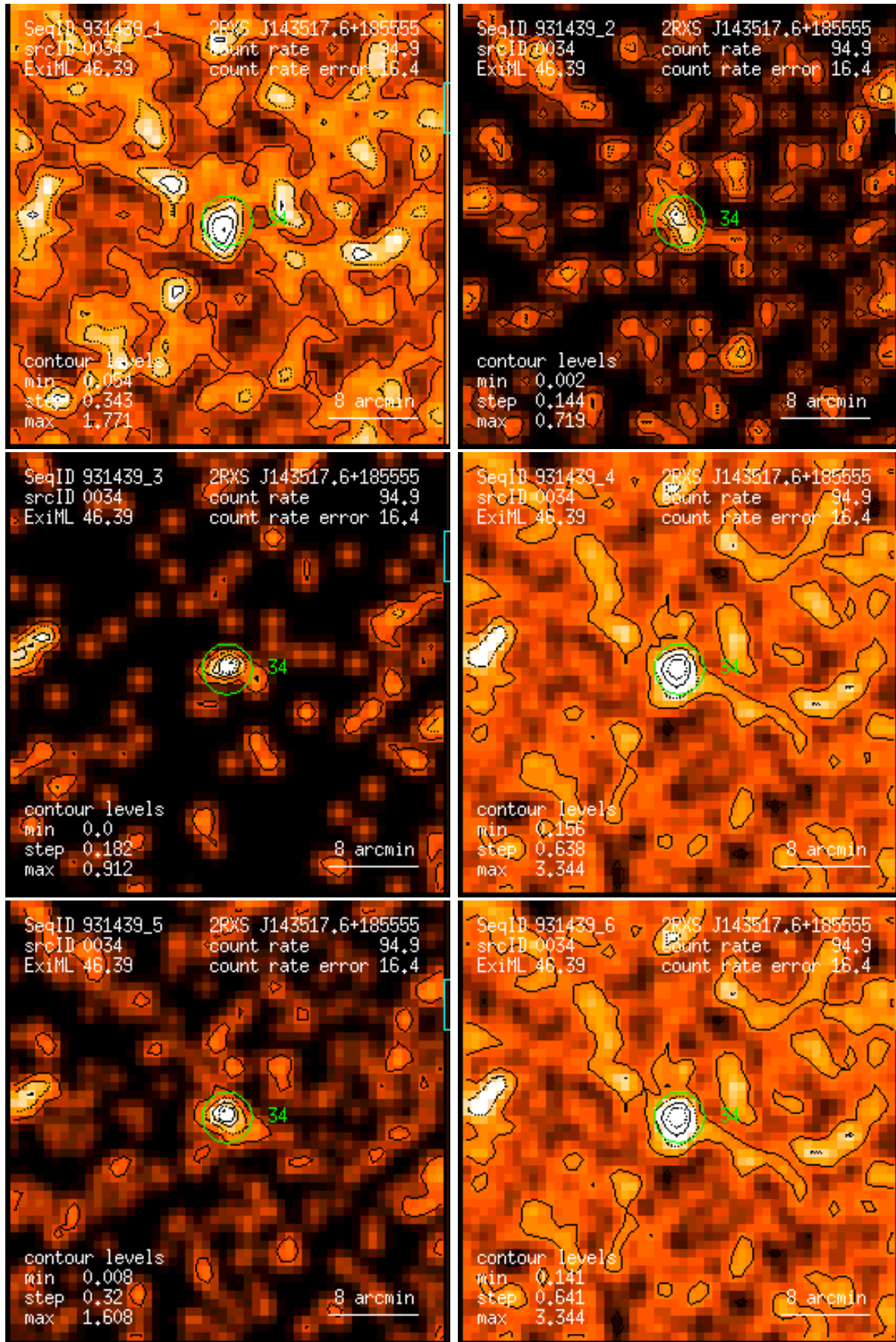
Figure 34: RASS 931439: detection 0034: band rate images, Gaussian filter: (1) PSPC channels 11 – 41, (2) 52 – 90, (3) 91 – 201, (4) 11 – 235, (5) 52 – 201, (6) 11 – 201. Broad band rates in counts/ks. Band rate contour levels in counts/ks/arcmin 2 .
