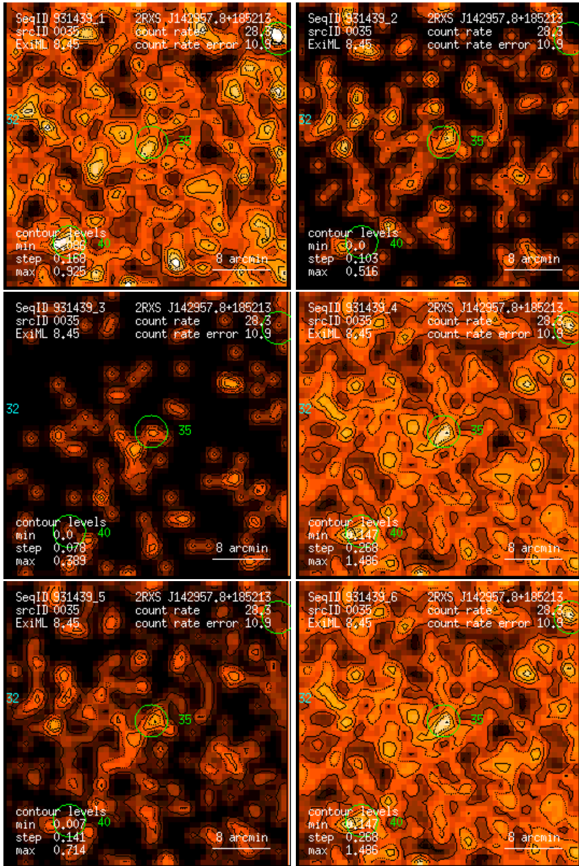
Figure 35: RASS 931439: detection 0035: band rate images, Gaussian filter: (1) PSPC channels 11 – 41, (2) 52 – 90, (3) 91 – 201, (4) 11 – 235, (5) 52 – 201, (6) 11 – 201. Broad band rates in counts/ks. Band rate contour levels in counts/ks/arcmin 2 .
