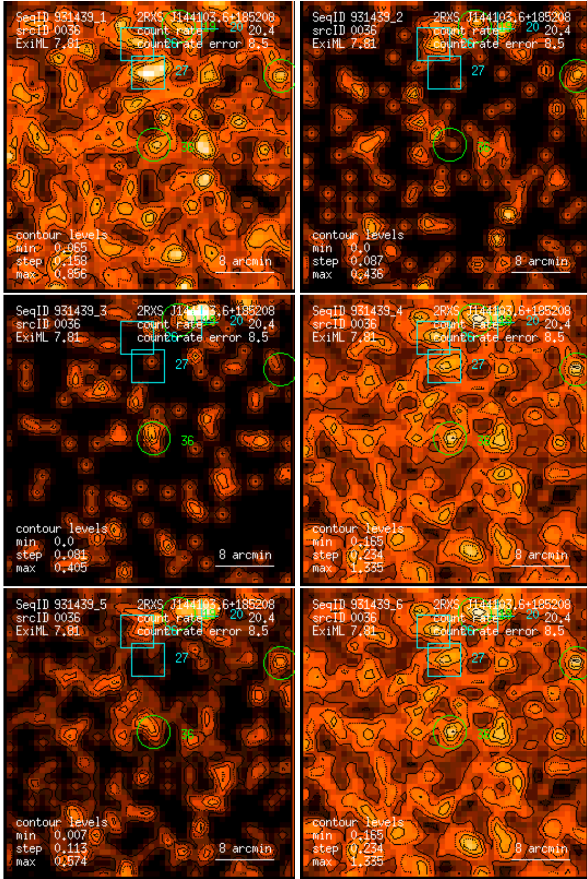
Figure 36: RASS 931439: detection 0036: band rate images, Gaussian filter: (1) PSPC channels 11 – 41, (2) 52 – 90, (3) 91 – 201, (4) 11 – 235, (5) 52 – 201, (6) 11 – 201. Broad band rates in counts/ks. Band rate contour levels in counts/ks/arcmin 2 .
