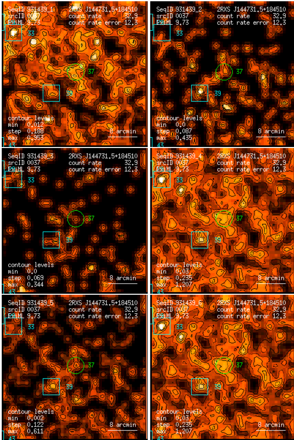
Figure 37: RASS 931439: detection 0037: band rate images, Gaussian filter: (1) PSPC channels 11 – 41, (2) 52 – 90, (3) 91 – 201, (4) 11 – 235, (5) 52 – 201, (6) 11 – 201. Broad band rates in counts/ks. Band rate contour levels in counts/ks/arcmin 2 .
