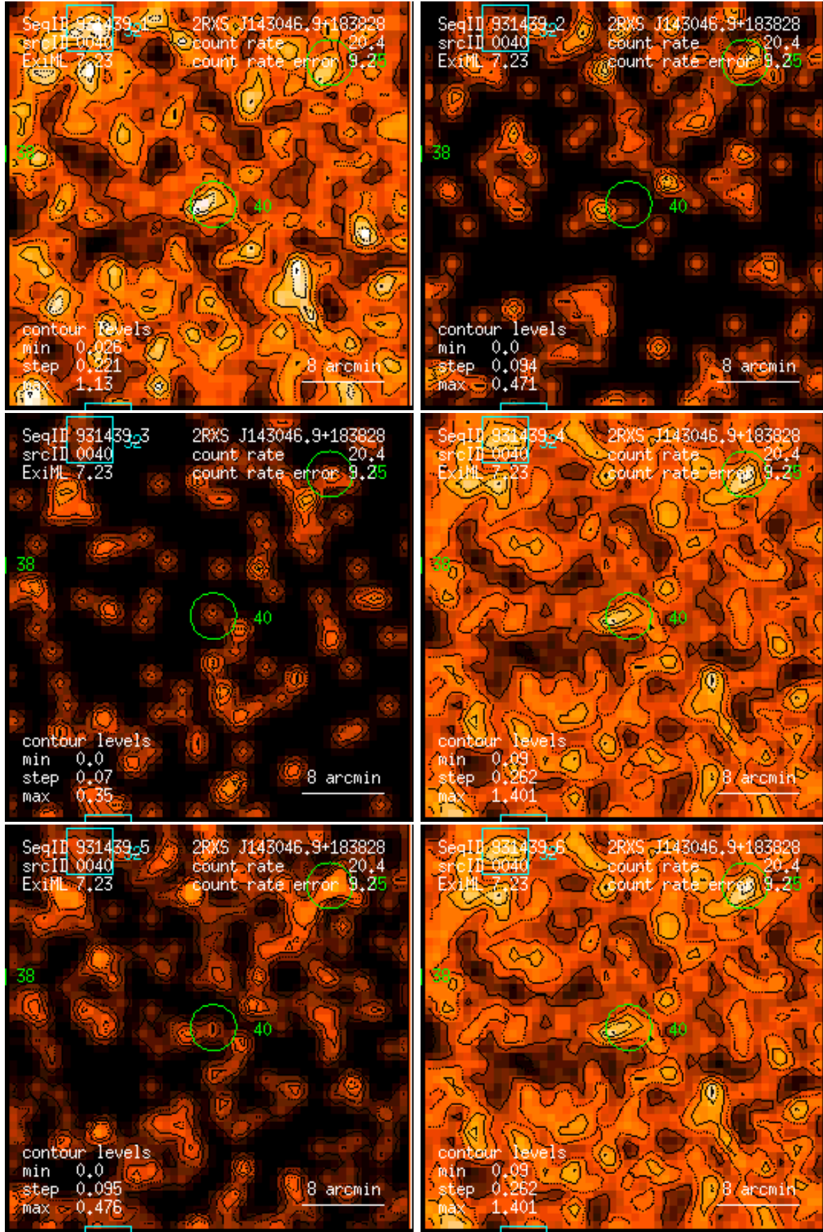
Figure 40: RASS 931439: detection 0040: band rate images, Gaussian filter: (1) PSPC channels 11 – 41, (2) 52 – 90, (3) 91 – 201, (4) 11 – 235, (5) 52 – 201, (6) 11 – 201. Broad band rates in counts/ks. Band rate contour levels in counts/ks/arcmin 2 .
