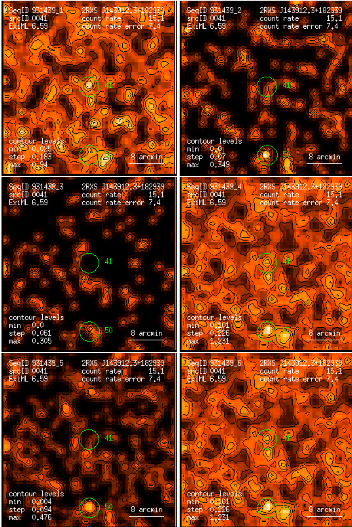
Figure 41: RASS 931439: detection 0041: band rate images, Gaussian filter: (1) PSPC channels 11 – 41, (2) 52 – 90, (3) 91 – 201, (4) 11 – 235, (5) 52 – 201, (6) 11 – 201. Broad band rates in counts/ks. Band rate contour levels in counts/ks/arcmin 2 .
