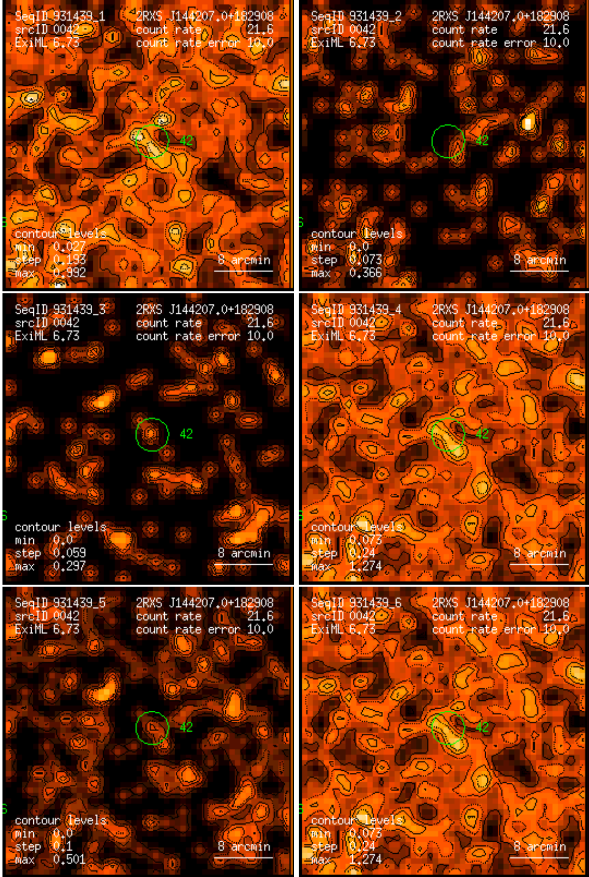
Figure 42: RASS 931439: detection 0042: band rate images, Gaussian filter: (1) PSPC channels 11 – 41, (2) 52 – 90, (3) 91 – 201, (4) 11 – 235, (5) 52 – 201, (6) 11 – 201. Broad band rates in counts/ks. Band rate contour levels in counts/ks/arcmin 2 .
