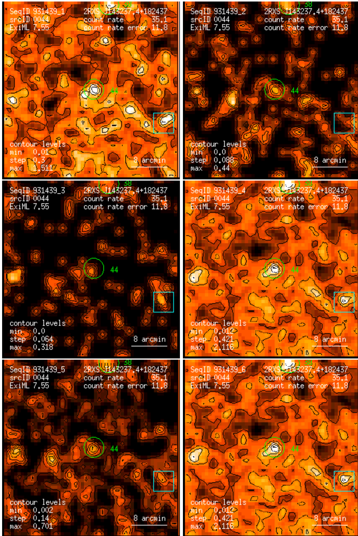
Figure 44: RASS 931439: detection 0044: band rate images, Gaussian filter: (1) PSPC channels 11 – 41, (2) 52 – 90, (3) 91 – 201, (4) 11 – 235, (5) 52 – 201, (6) 11 – 201. Broad band rates in counts/ks. Band rate contour levels in counts/ks/arcmin 2 .
