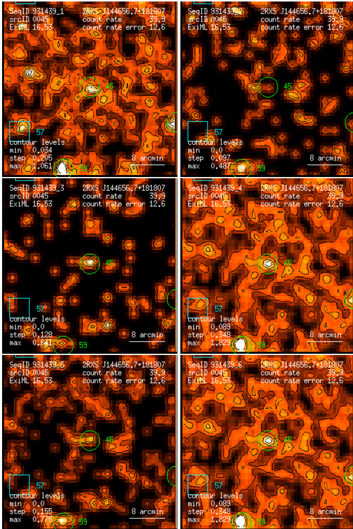
Figure 45: RASS 931439: detection 0045: band rate images, Gaussian filter: (1) PSPC channels 11 – 41, (2) 52 – 90, (3) 91 – 201, (4) 11 – 235, (5) 52 – 201, (6) 11 – 201. Broad band rates in counts/ks. Band rate contour levels in counts/ks/arcmin 2 .
