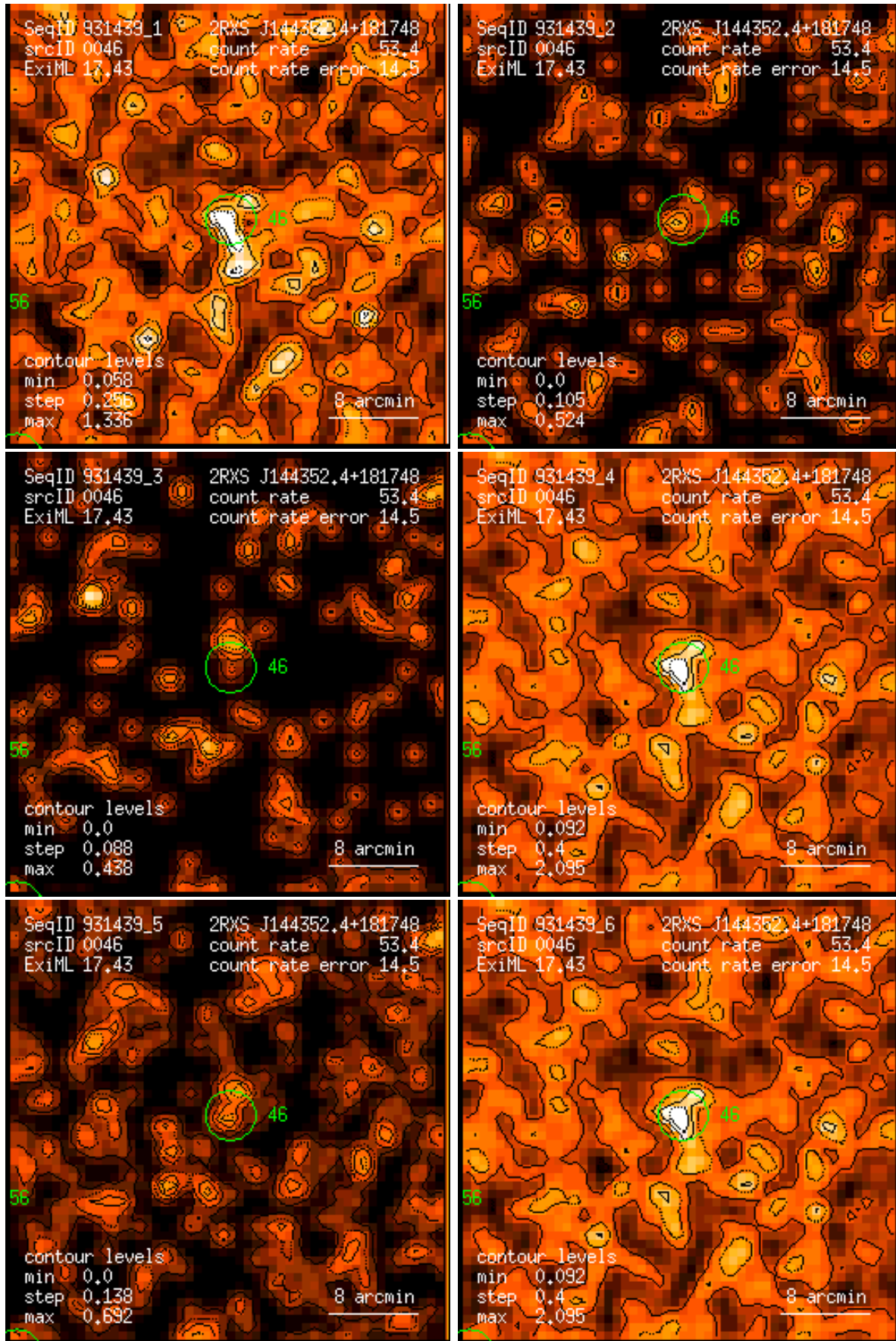
Figure 46: RASS 931439: detection 0046: band rate images, Gaussian filter: (1) PSPC channels 11 – 41, (2) 52 – 90, (3) 91 – 201, (4) 11 – 235, (5) 52 – 201, (6) 11 – 201. Broad band rates in counts/ks. Band rate contour levels in counts/ks/arcmin 2 .
