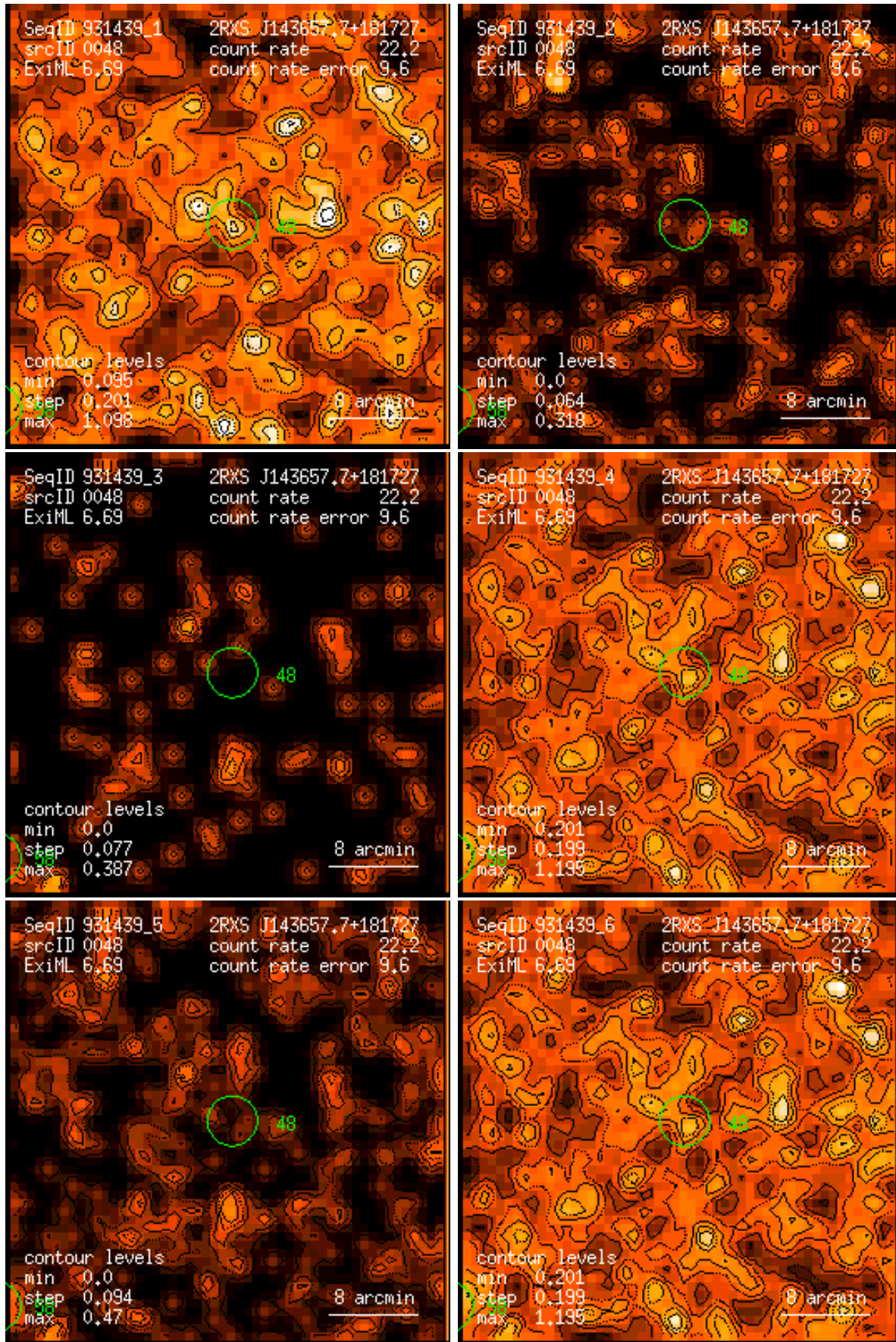
Figure 48: RASS 931439: detection 0048: band rate images, Gaussian filter: (1) PSPC channels 11 – 41, (2) 52 – 90, (3) 91 – 201, (4) 11 – 235, (5) 52 – 201, (6) 11 – 201. Broad band rates in counts/ks. Band rate contour levels in counts/ks/arcmin 2 .
