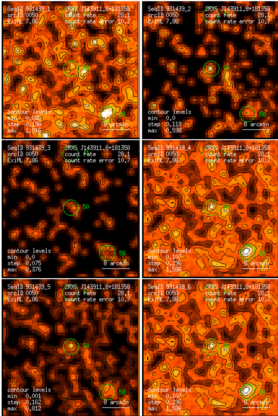
Figure 50: RASS 931439: detection 0050: band rate images, Gaussian filter: (1) PSPC channels 11 – 41, (2) 52 – 90, (3) 91 – 201, (4) 11 – 235, (5) 52 – 201, (6) 11 – 201. Broad band rates in counts/ks. Band rate contour levels in counts/ks/arcmin 2 .
