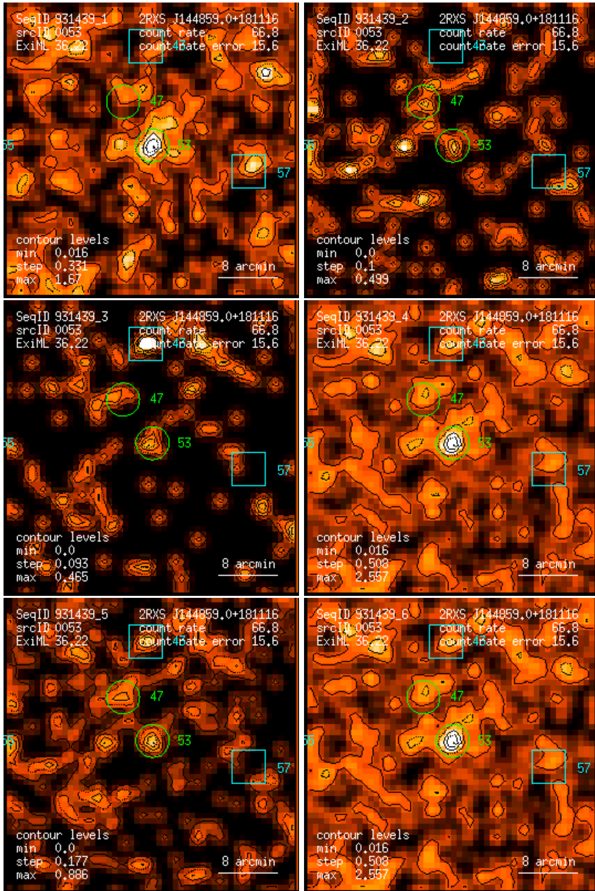
Figure 53: RASS 931439: detection 0053: band rate images, Gaussian filter: (1) PSPC channels 11 – 41, (2) 52 – 90, (3) 91 – 201, (4) 11 – 235, (5) 52 – 201, (6) 11 – 201. Broad band rates in counts/ks. Band rate contour levels in counts/ks/arcmin 2 .
