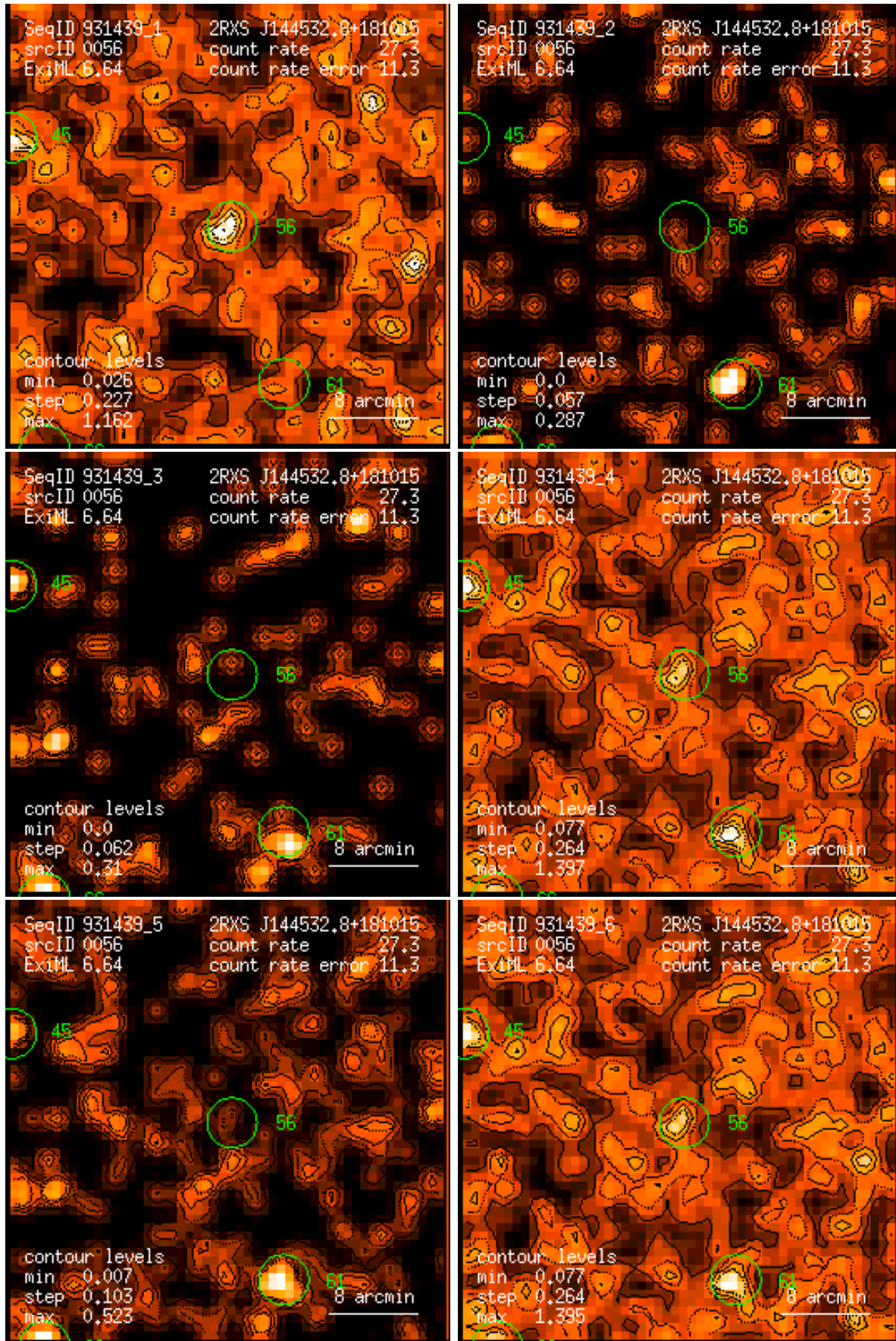
Figure 56: RASS 931439: detection 0056: band rate images, Gaussian filter: (1) PSPC channels 11 – 41, (2) 52 – 90, (3) 91 – 201, (4) 11 – 235, (5) 52 – 201, (6) 11 – 201. Broad band rates in counts/ks. Band rate contour levels in counts/ks/arcmin 2 .
