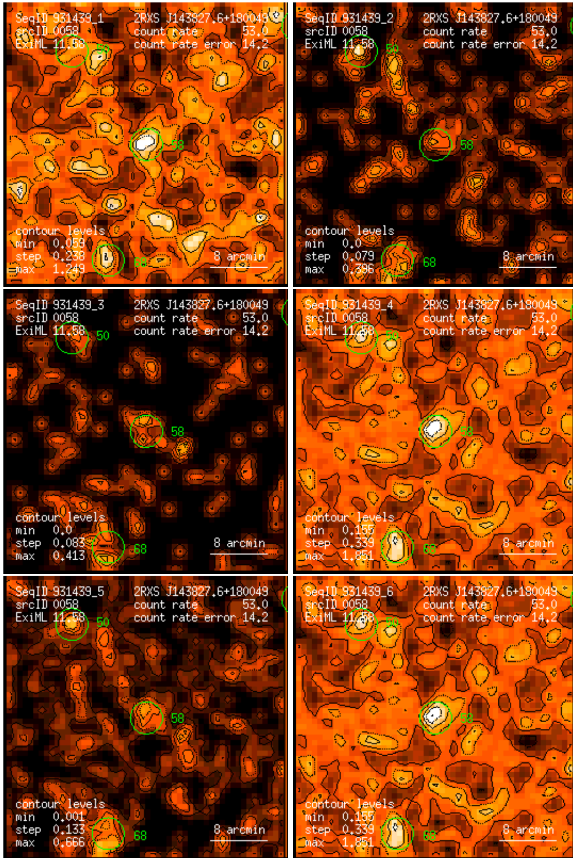
Figure 58: RASS 931439: detection 0058: band rate images, Gaussian filter: (1) PSPC channels 11 – 41, (2) 52 – 90, (3) 91 – 201, (4) 11 – 235, (5) 52 – 201, (6) 11 – 201. Broad band rates in counts/ks. Band rate contour levels in counts/ks/arcmin 2 .
