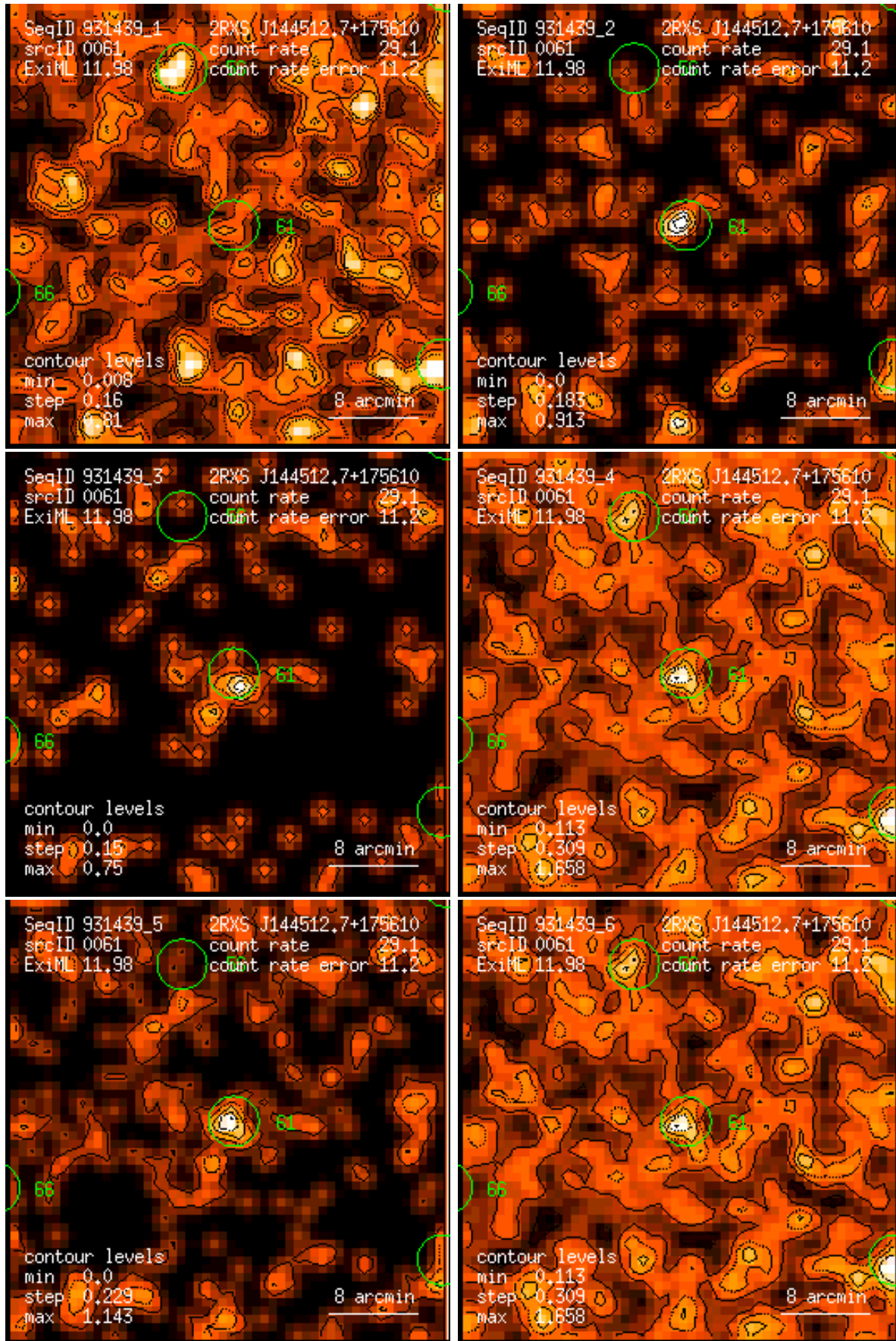
Figure 61: RASS 931439: detection 0061: band rate images, Gaussian filter: (1) PSPC channels 11 – 41, (2) 52 – 90, (3) 91 – 201, (4) 11 – 235, (5) 52 – 201, (6) 11 – 201. Broad band rates in counts/ks. Band rate contour levels in counts/ks/arcmin 2 .
