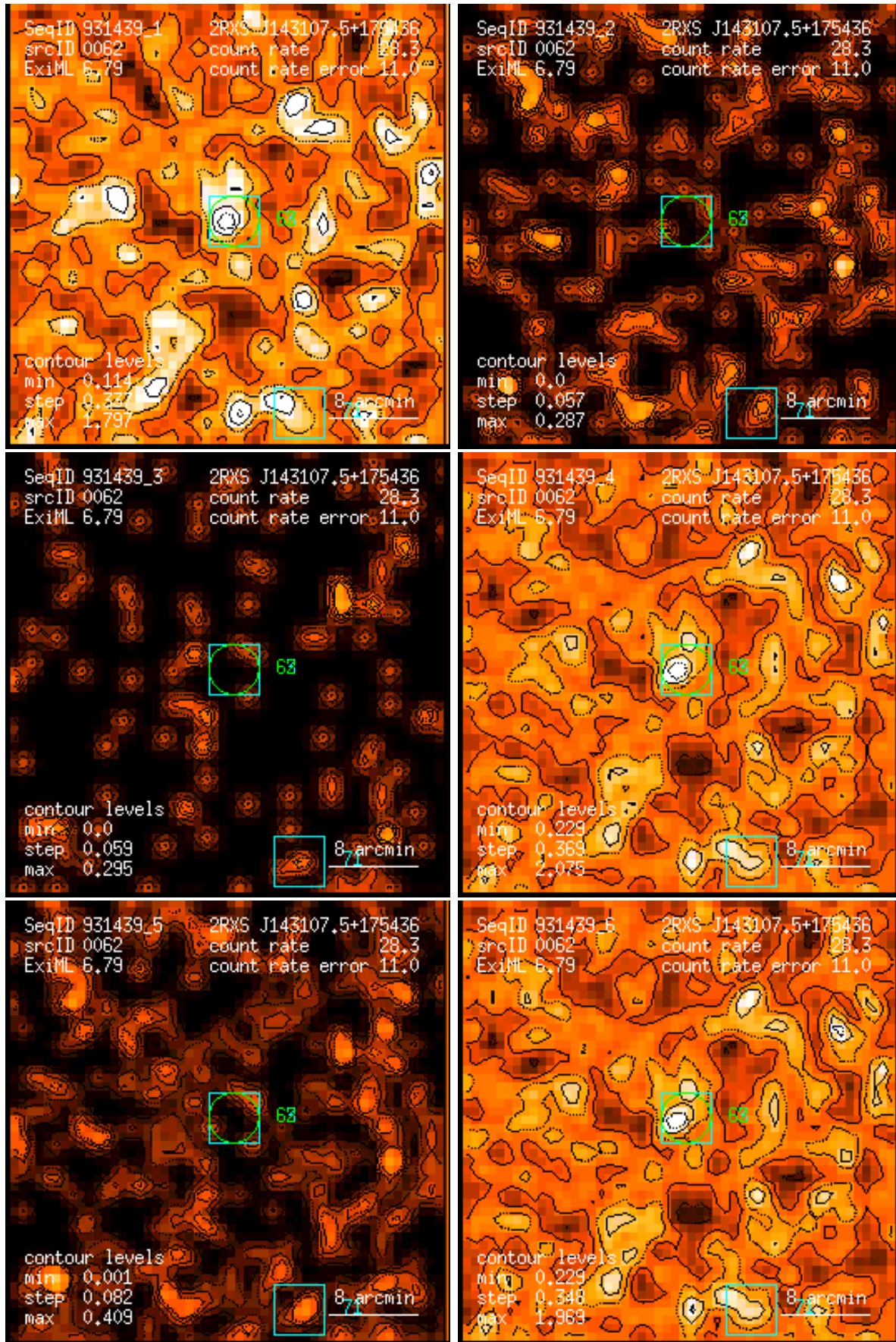
Figure 62: RASS 931439: detection 0062: band rate images, Gaussian filter: (1) PSPC channels 11 – 41, (2) 52 – 90, (3) 91 – 201, (4) 11 – 235, (5) 52 – 201, (6) 11 – 201. Broad band rates in counts/ks. Band rate contour levels in counts/ks/arcmin 2 .
